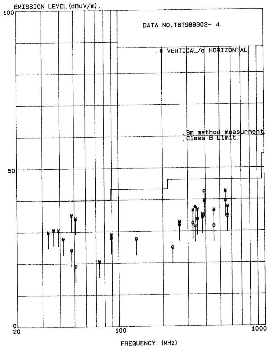
Figure 6.2-2 RFI Field Strength Measurement Results
