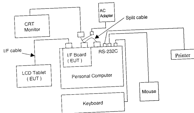
Figure 4-1 System Configuration Diagram
