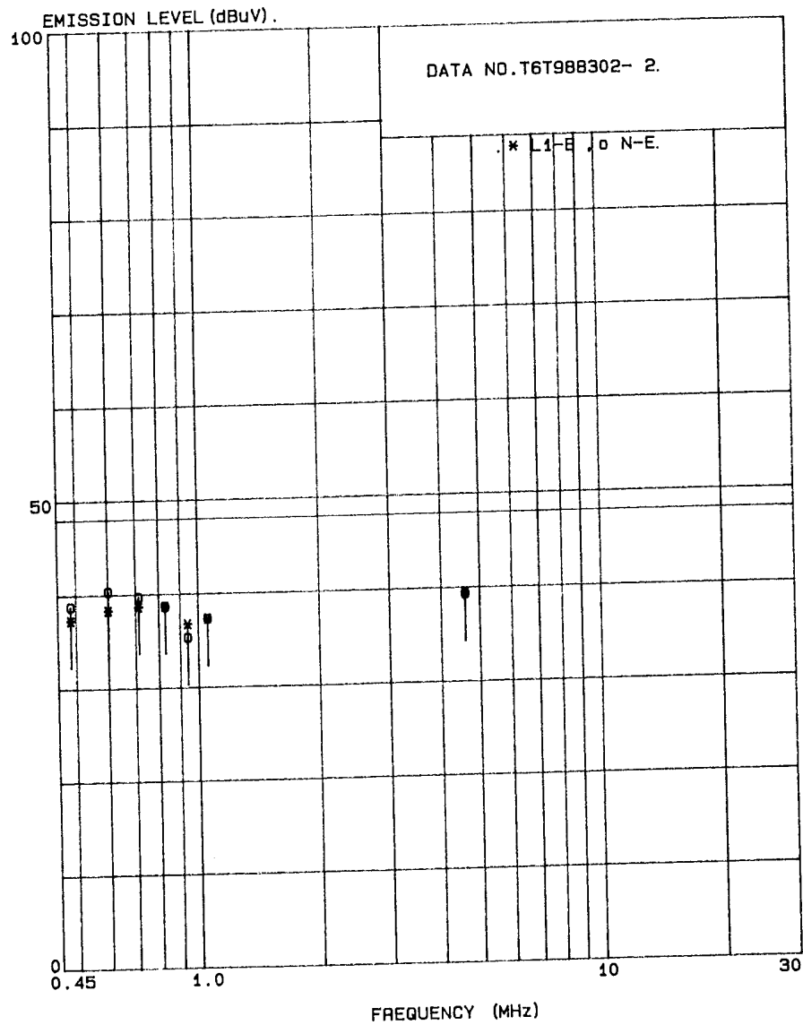
Figure 6.1-2 RFI Voltage Measurement Results
