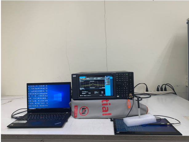
P15.221+RSS-Gen_EMR_Radiated_Setup
