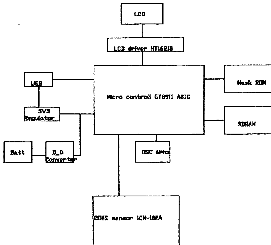
Block Diagram of D-cam
