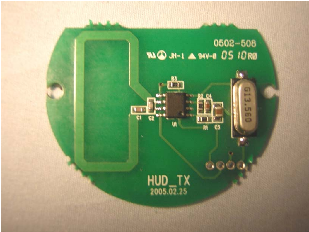
RF board with antenna etched on it
