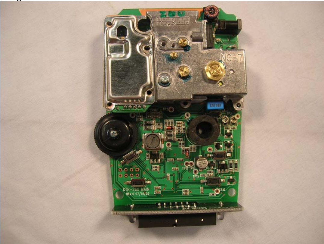
Top with shield on daughter card
