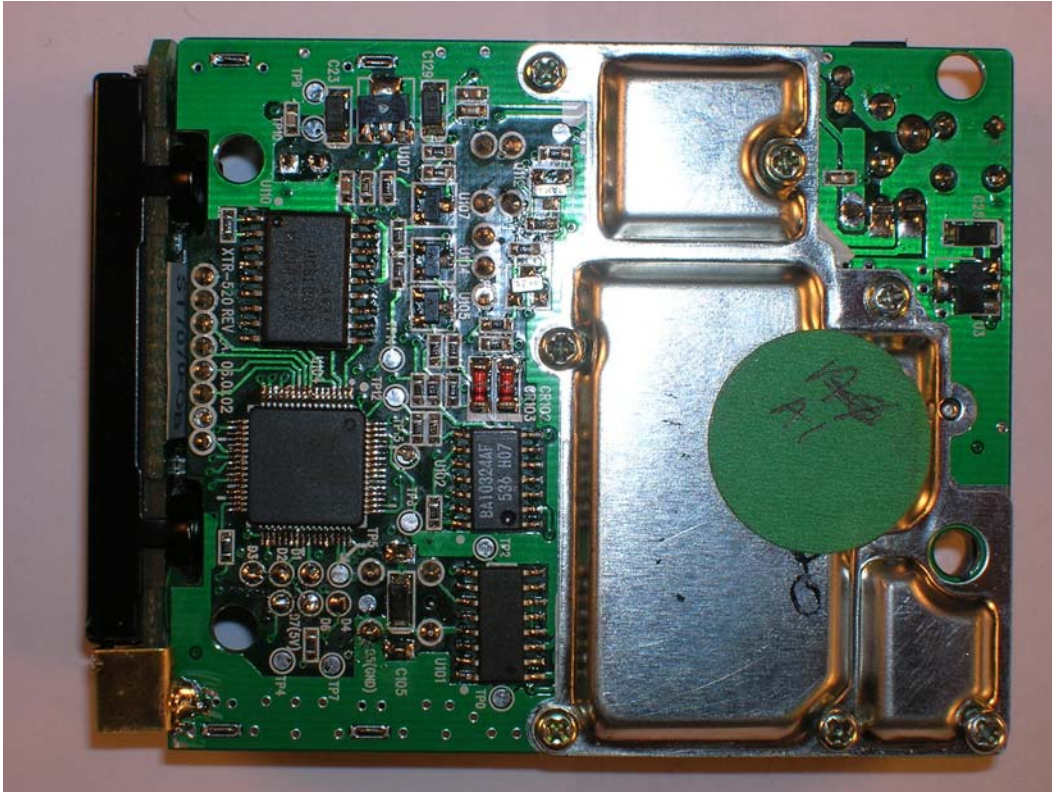
XTR-520 PCB bottom view
