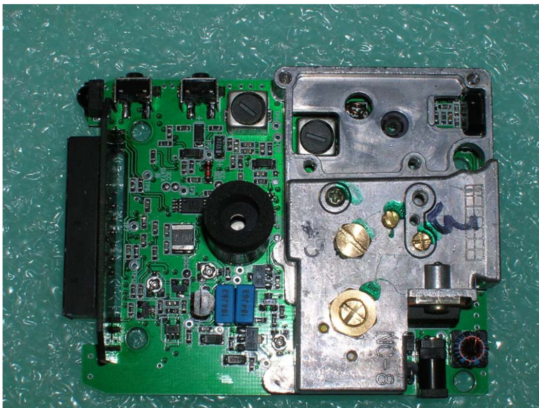
XTR-220 PCB top view
