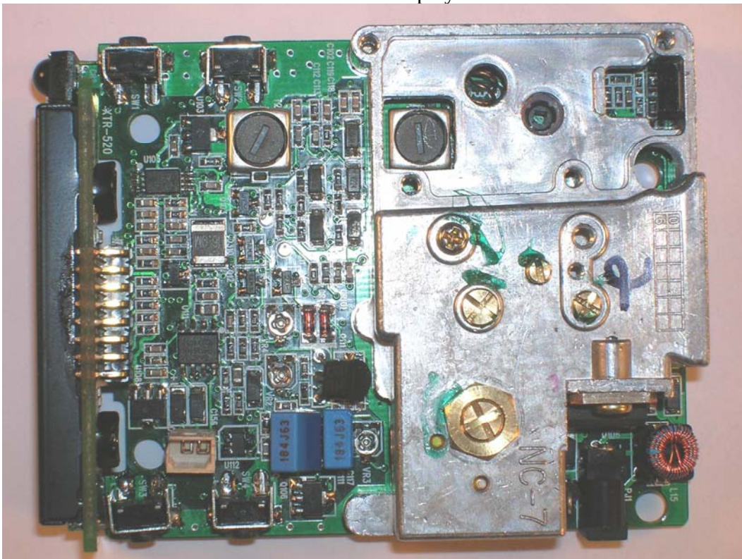
XTR-520 PCB top view
