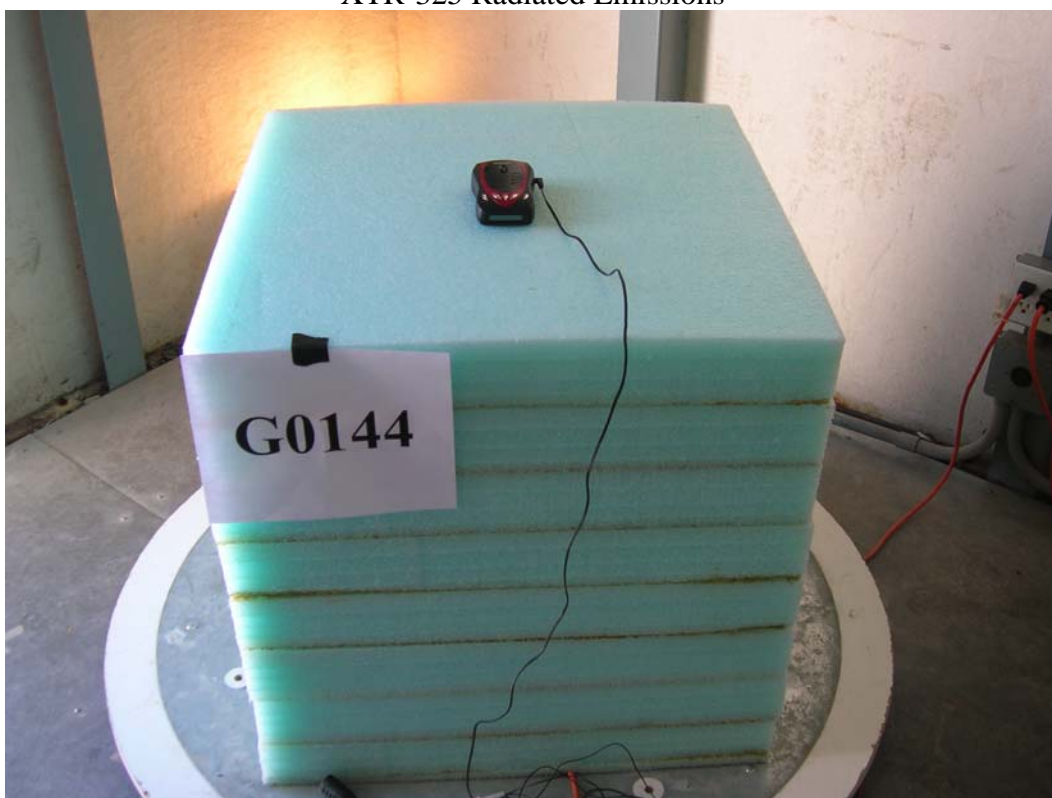
XTR-425 Radiated Emissions
