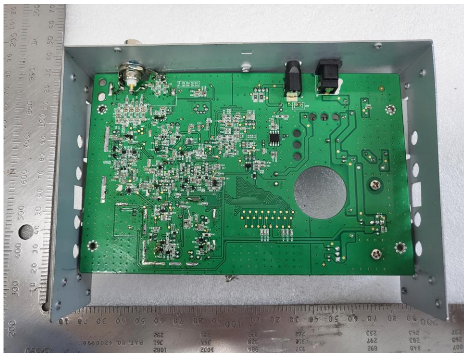
Front View of Sub Board 1
