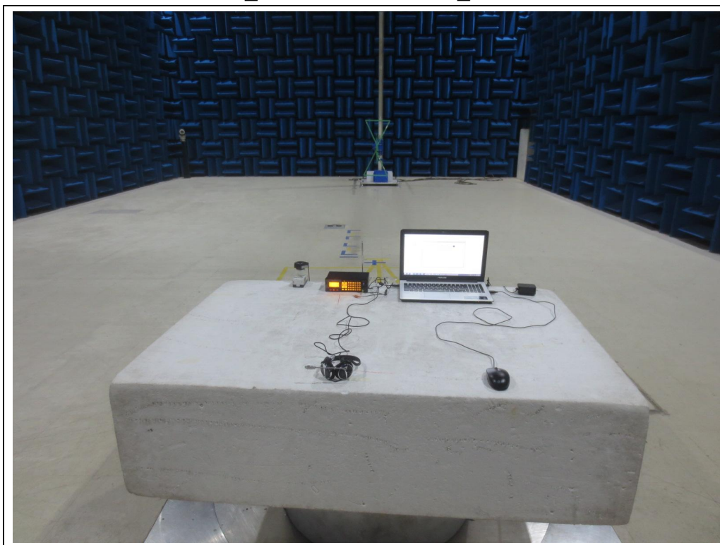
WS1065 _ < 30 MHz ~ 1 GHz _ MODE 2 >
