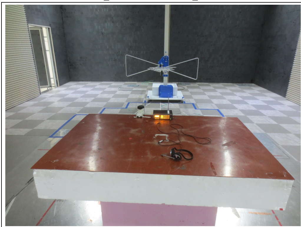
PRO-652 _ < 30 MHz ~ 1 GHz _ MODE 1 >
