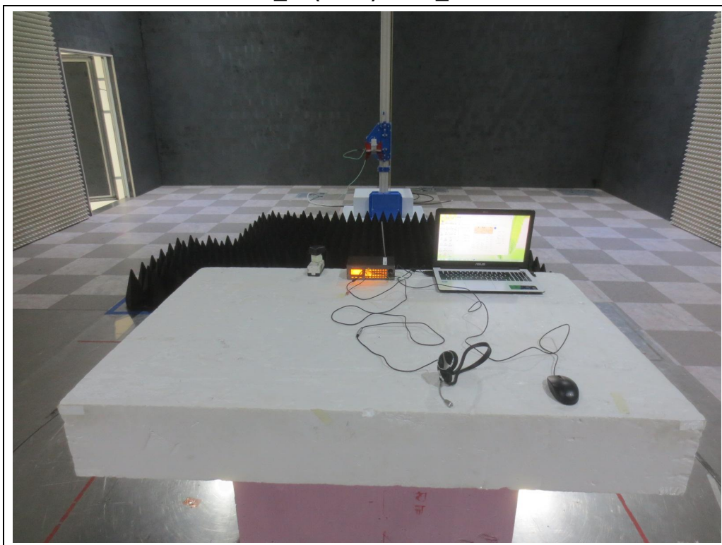
PRO-652 _ < (1 ~ 6) GHz _ MODE 2 >
