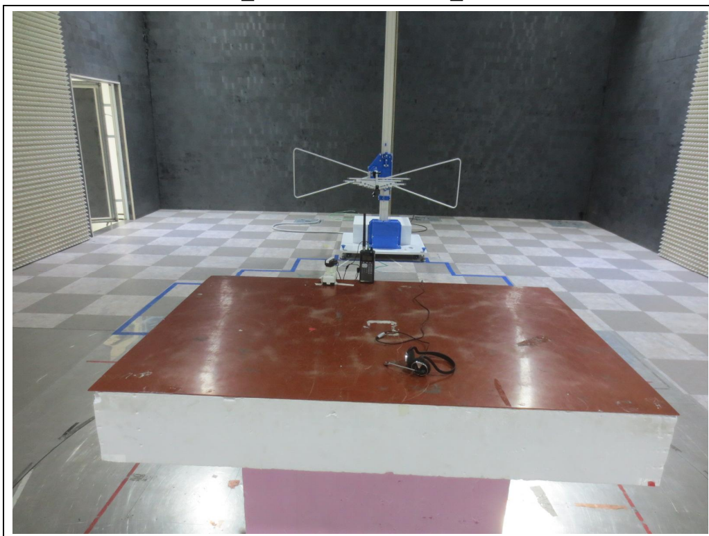
PRO-651_ < 30 MHz ~ 1 GHz _ MODE 1 >
