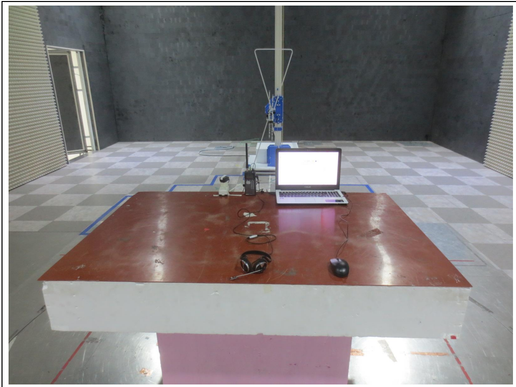
PRO-651_ < 30 MHz ~ 1 GHz _ MODE 2 >
