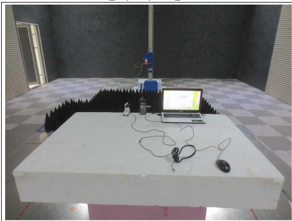
PRO-651_ < (1 ~ 6) GHz _ MODE 2 >
