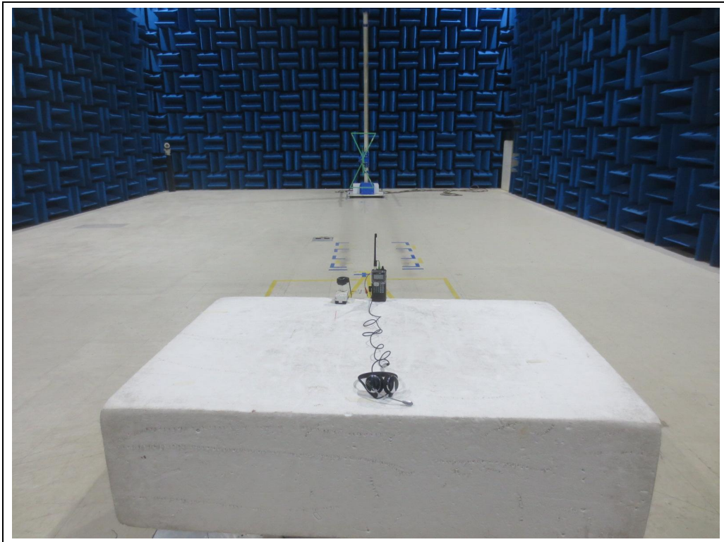
WS1040 _ < 30 MHz ~ 1 GHz _ MODE 1 >
