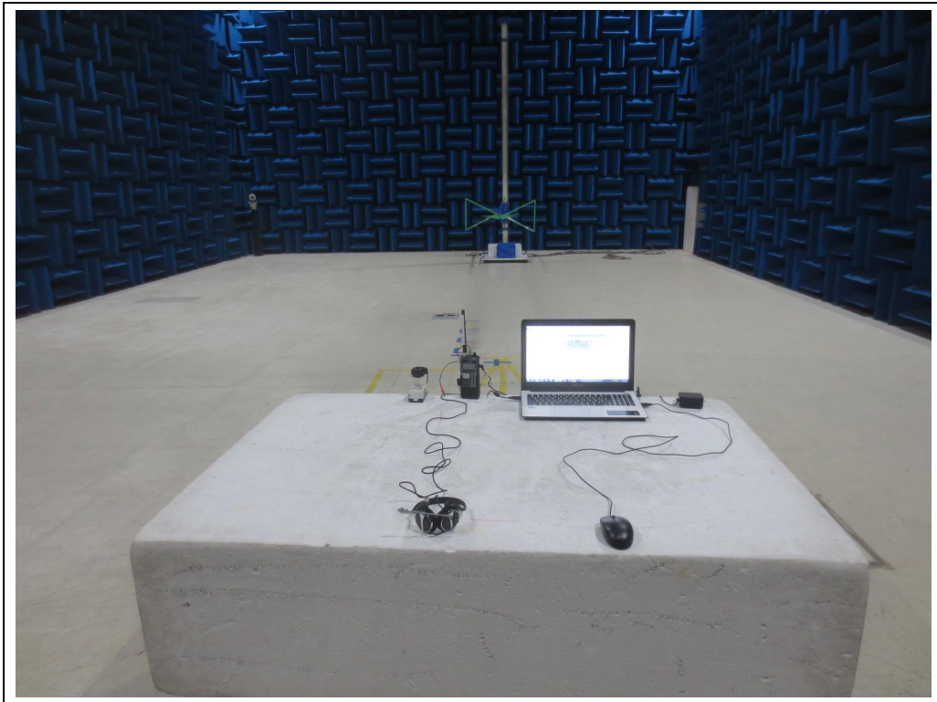
WS1040 _ < 30 MHz ~ 1 GHz _ MODE 2 >
