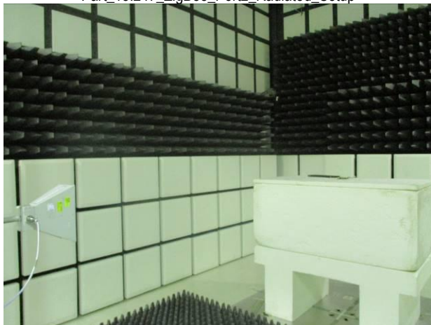
Part_15.247_ZigBee_Port2_Radiated_Setup
