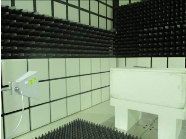
Part_15.247_2.4G_Radiated_Dipole_Setup
