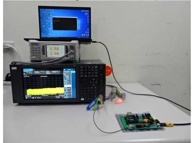
Part_15.247_ZigBee_Port2_Conducted_Setup
