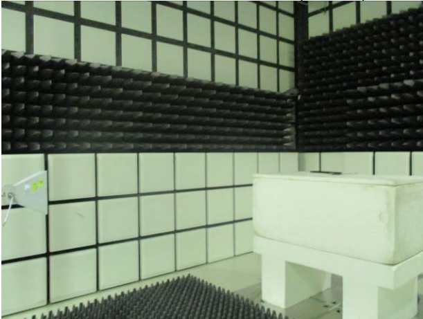
Part 15.247 LE_Port1_Radiated_monopole_Setup
