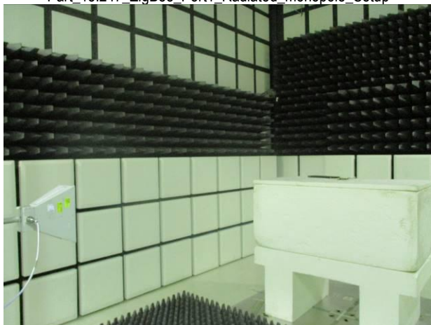
Part 15.247 ZigBee_Port1 Radiated monopole Setup
