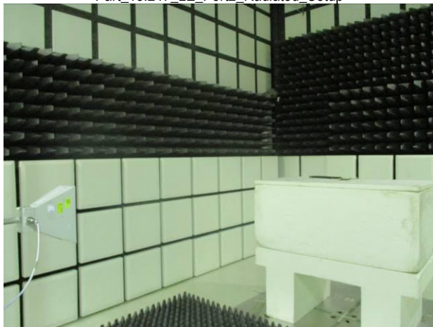
Part_15.247_LE_Port2_Radiated_Setup
