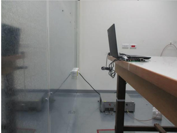
Part_15.247_ZigBee_Conduction_Setup
