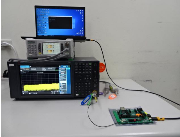
Part_15.247_LE_Port1_Conducted_Setup
