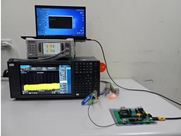
Part_15.247_LE_Port2_Conducted_Setup
