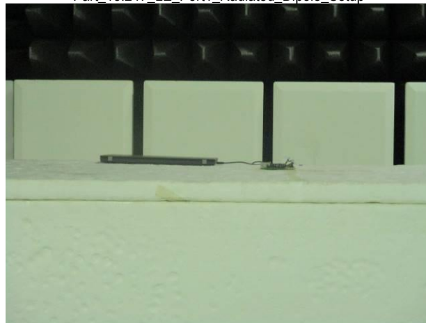
Part_15.247_LE_Port1_Radiated_Dipole_Setup
