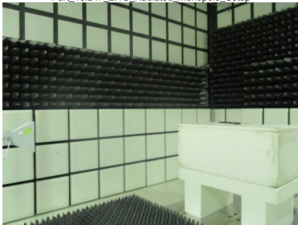
Part_15.247_2.4G_Radiated_Monopole_Setup
