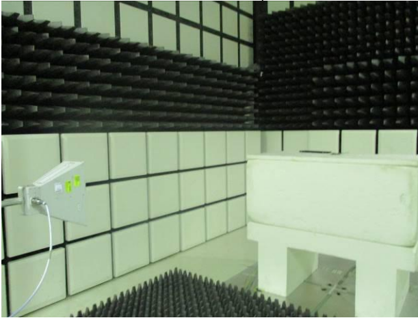
Co-Location_Setup
