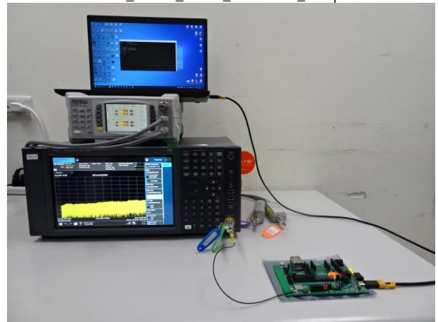
Part_15.407_WLAN_Conducted_Setup
