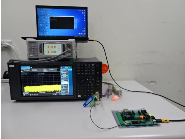
Part_15.247_LE_Port2_Conducted_Setup
