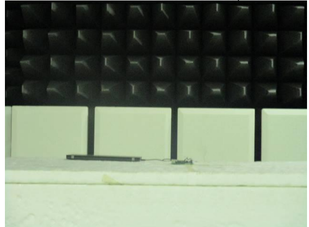
Part 15.247 LE_Port2_Radiated_Setup
