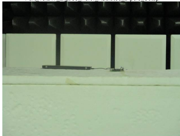
Part_15.247_ZigBee_Port1_Radiated_Dipole_Setup
