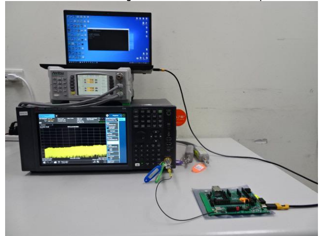
Part_15.407_WLAN_Conducted_Setup
