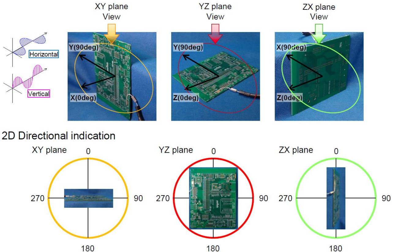
Figure 10: Antenna Measurement Directions (Japan)
