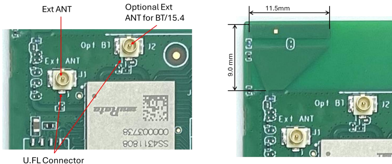
Figure 5: EVB Design Used for Testing
