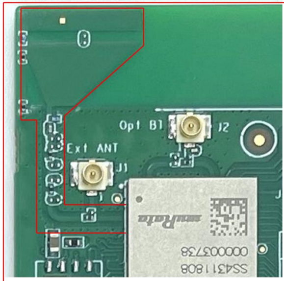
Figure 8: Trace antenna (Type 2FR_Antenna) Layout Guide
