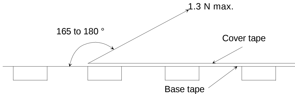
Figure 11.5 Peeling Force Diagram
