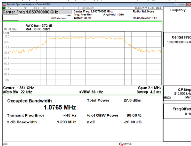
Band25_1.4MHz_Chain0_1850.7MHz_NBI 0_16QAM_6_0
