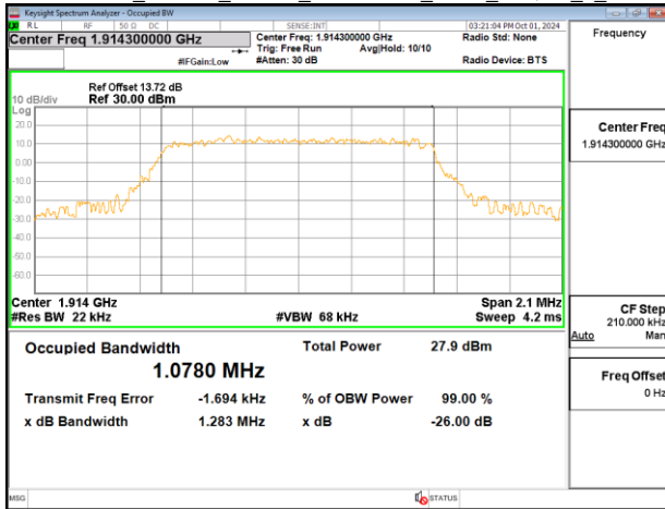
Band25_1.4MHz_Chain0_1914.3MHz_NBI 0_QPSK_6_0
