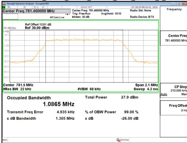
Band13_10MHz_Chain0_782MHz_NBI 3_QPSK_6_0
