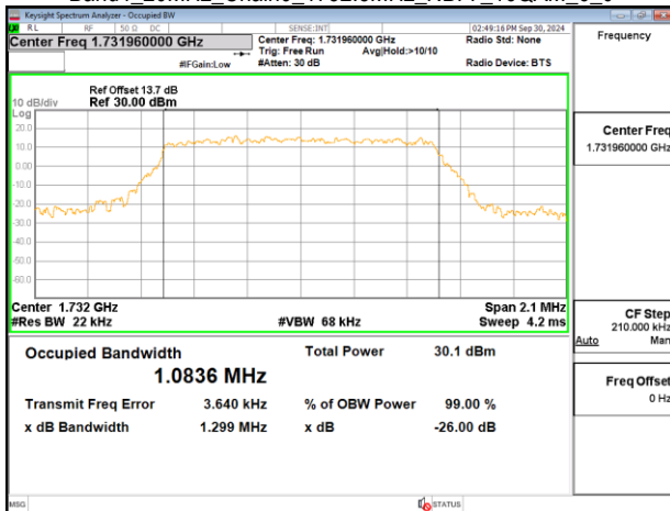
Band4_20MHz_Chain0_1732.5MHz_NBI 7_16QAM_6_0
