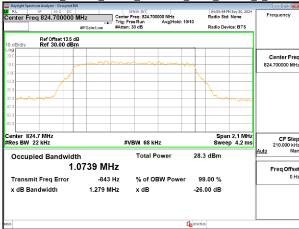
Band5_1.4MHz_Chain0_824.7MHz_NBI 0_QPSK_6_0
