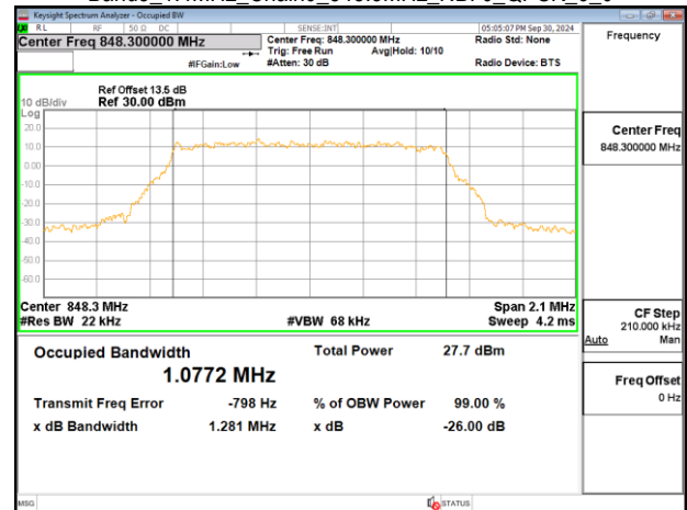
Band5_1.4MHz_Chain0_848.3MHz_NBI 0_QPSK_6_0
