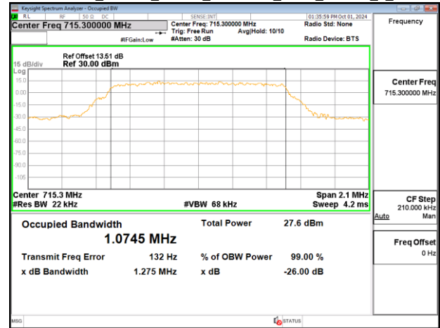
Band12_1.4MHz_Chain0_715.3MHz_NBI_0_QPSK_6_0
