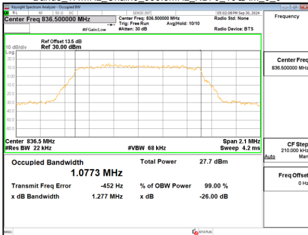
Band5_1.4MHz_Chain0_836.5MHz_NBI 0_16QAM_6_0
