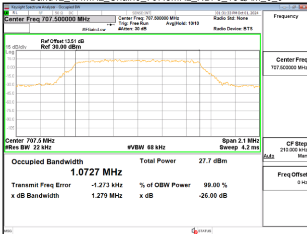
Band12_1.4MHz_Chain0_707.5MHz_NBI_0_16QAM_6_0
