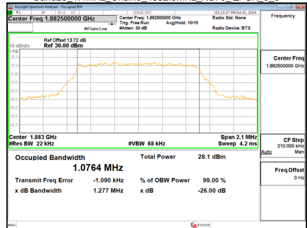
Band25_1.4MHz_Chain0_1882.5MHz_NBI 0_QPSK_6_0
