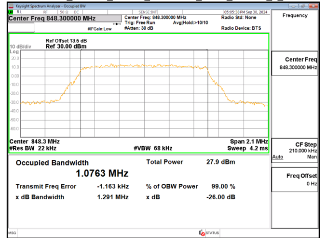
Band5_1.4MHz_Chain0_848.3MHz_NBI 0_QPSK_6_0
