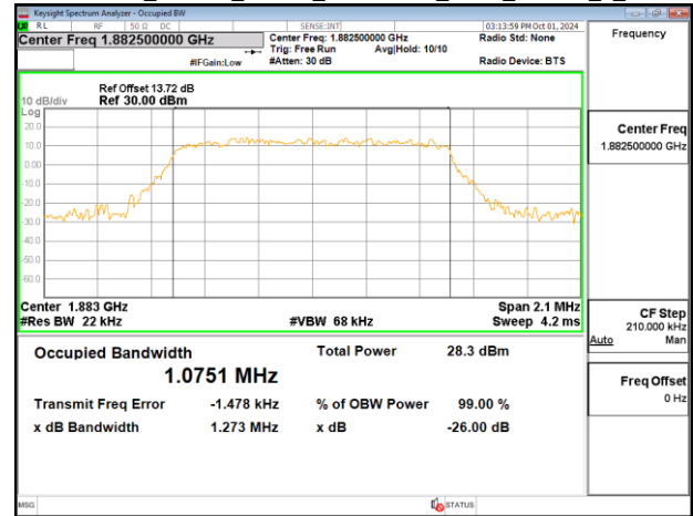
Band25_1.4MHz_Chain0_1882.5MHz_NBI 0_QPSK_6_0
