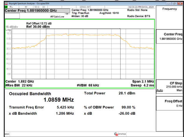
Band25_10MHz_Chain0_1882.5MHz_NBI 3_QPSK_6_0
