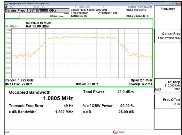
Band25_5MHz_Chain0_1882.5MHz_NBI 1_QPSK_6_0
