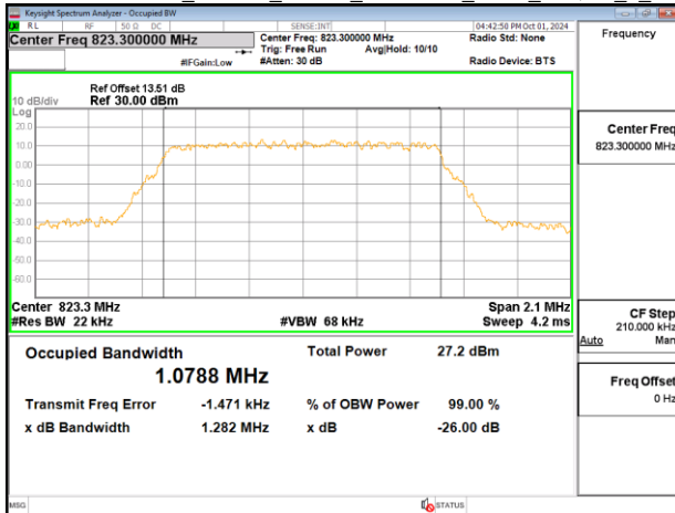
Band26-Part90s_1.4MHz_Chain0_823.3MHz_NBI_0_QPSK_6_0
