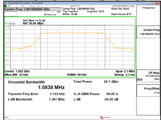
Band25_20MHz_Chain0_1882.5MHz_NBI 7_QPSK_6_0
