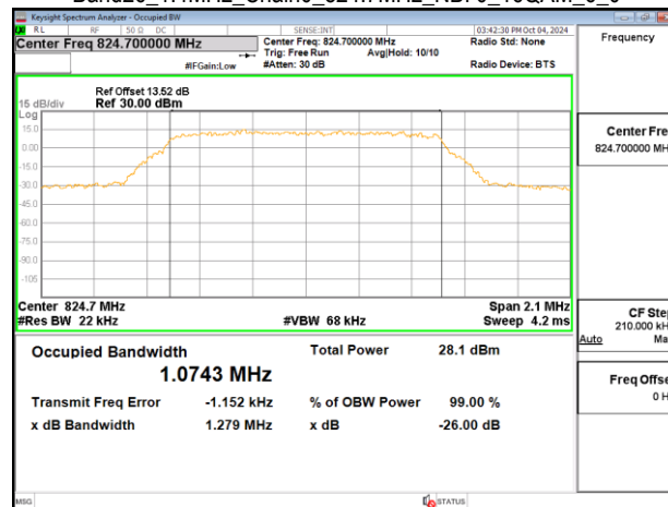
Band26_1.4MHz_Chain0_824.7MHz_NBI 0_QPSK_6_0
