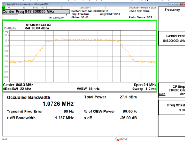
Band26 1.4MHz_Chain0 848.3MHz_NBI 0_16QAM 6 0
