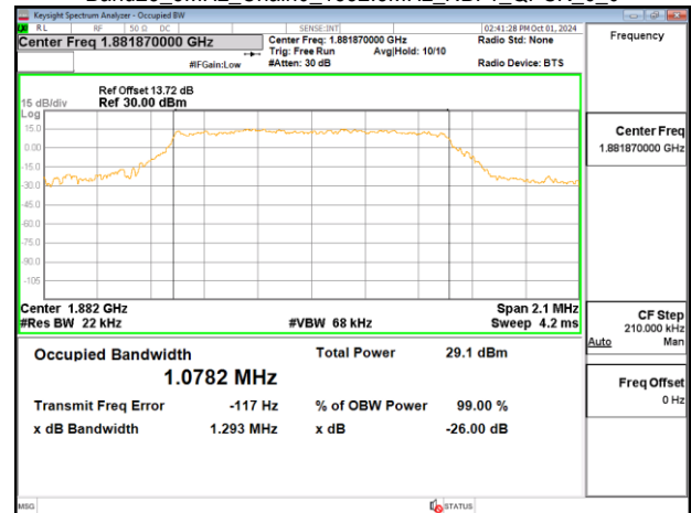
Band25_5MHz_Chain0_1882.5MHz_NBI 1_QPSK_6_0
