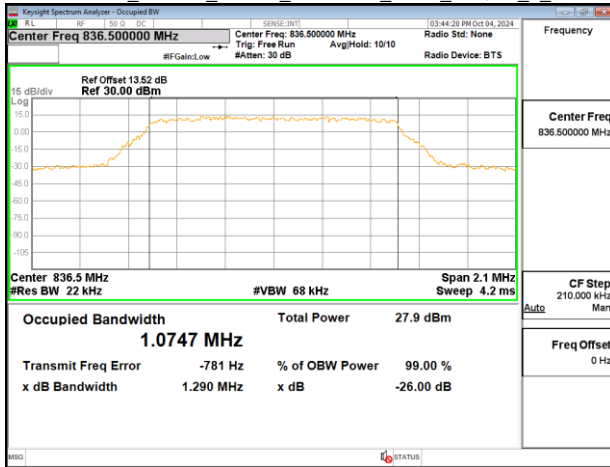
Band26 1.4MHz_Chain0 836.5MHz_NBI 0_QPSK 6 0
