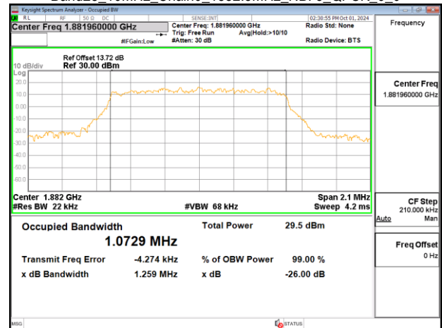
Band25_10MHz_Chain0_1882.5MHz_NBI 3_QPSK_6_0
