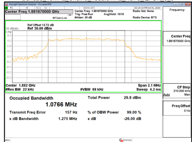
Band25_15MHz_Chain0_1882.5MHz_NBI 5_QPSK_6_0
