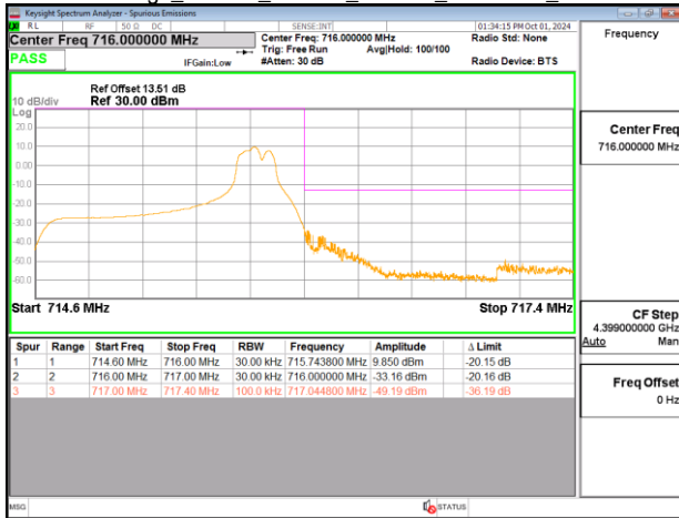
Band Edge_Band12_1.4MHz_PUSCH_715.3MHz_Chain0
