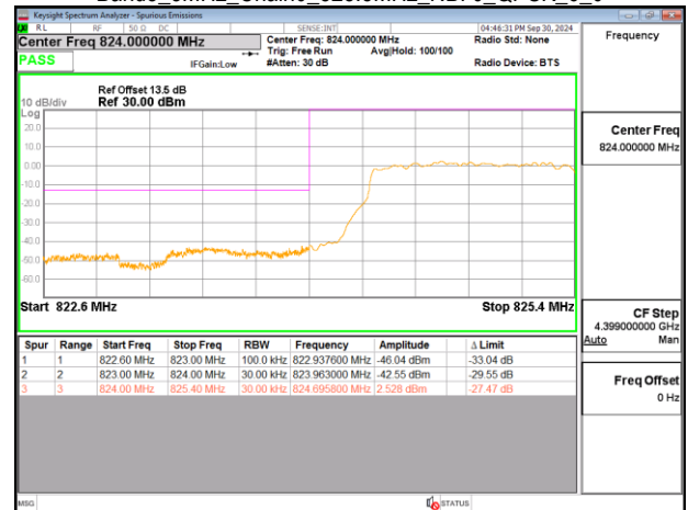
Band5_3MHz_Chain0_825.5MHz_NBI_0_QPSK_6_0
