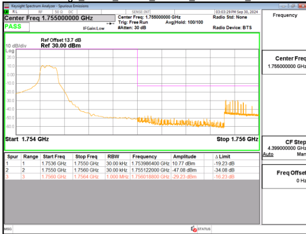
Band Edge_Band4_15MHz_PUSCH_1747.5MHz_Chain0
