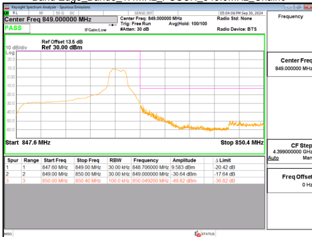
Band Edge_Band5_1.4MHz_PUSCH_848.3MHz_Chain0
