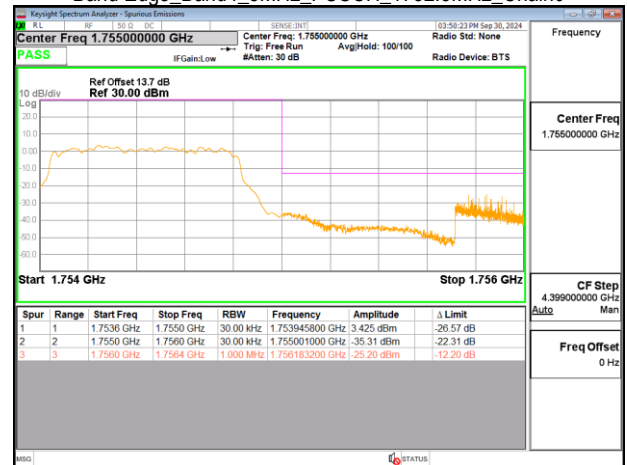
Band Edge_Band4_5MHz_PUSCH_1752.5MHz_Chain0
