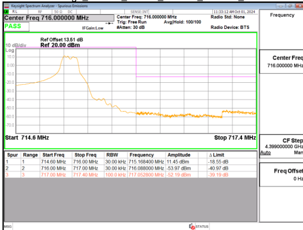
Band Edge_Band12_10MHz_PUSCH_711MHz_Chain0
