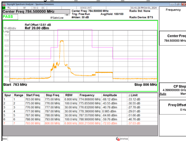
Band Edge_Band13_10MHz_PUSCH_782MHz_Chain0
