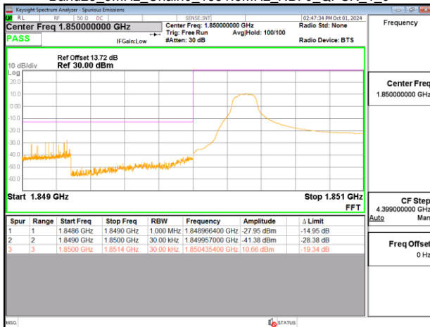
Band25_3MHz_Chain0_1851.5MHz_NBI 0_QPSK 1_0
