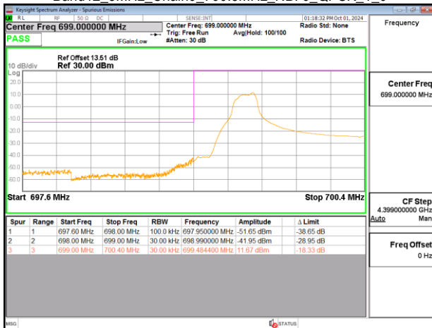
Band12_3MHz_Chain0_700.5MHz_NBI 0_QPSK_1_0
