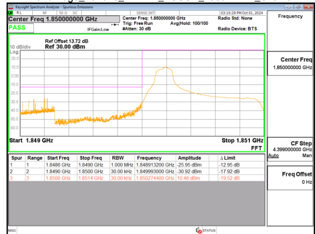
Band Edge_Band25_1.4MHz_PUSCH_1850.7MHz_Chain0
