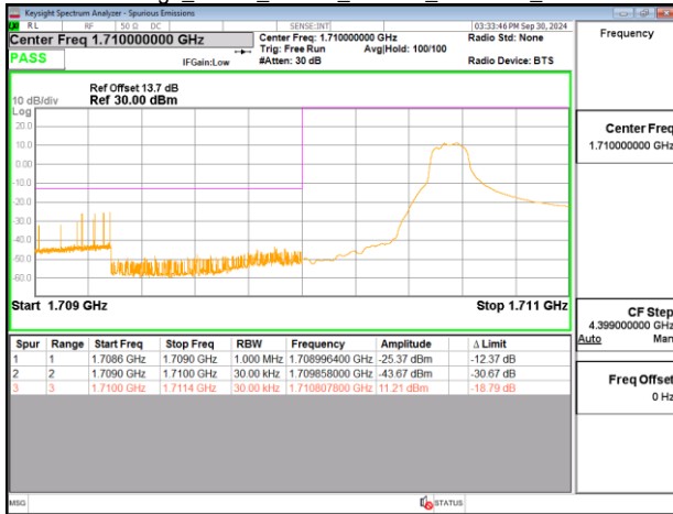
Band Edge_Band4_10MHz_PUSCH_1715MHz_Chain0
