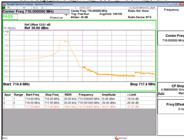
Band Edge_Band12_5MHz_PUSCH_713.5MHz_Chain0
