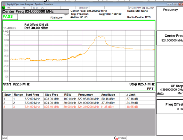
Band Edge_Band5_5MHz_PUSCH_826.5MHz_Chain0
