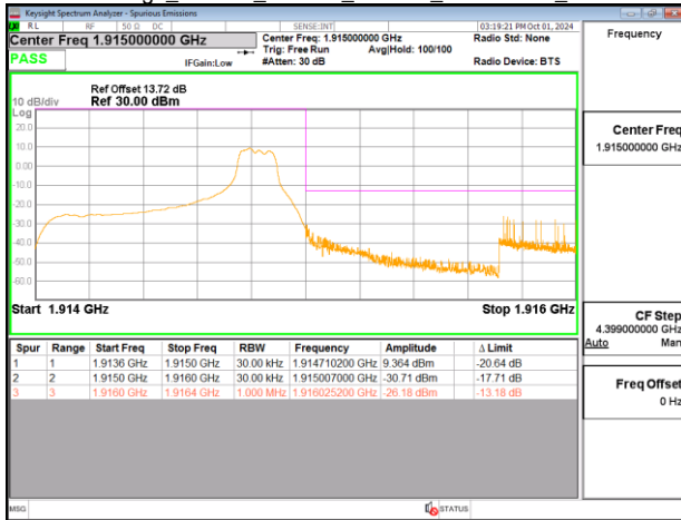
Band Edge_Band25_1.4MHz_PUSCH_1914.3MHz_Chain0
