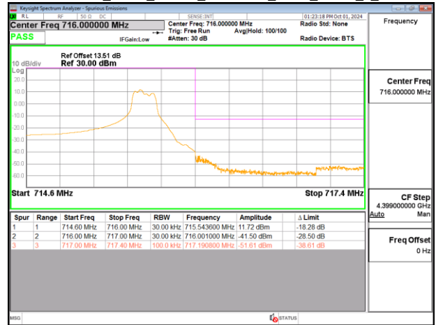
Band12_3MHz_Chain0_714.5MHz_NBI 1_QPSK_6_0
