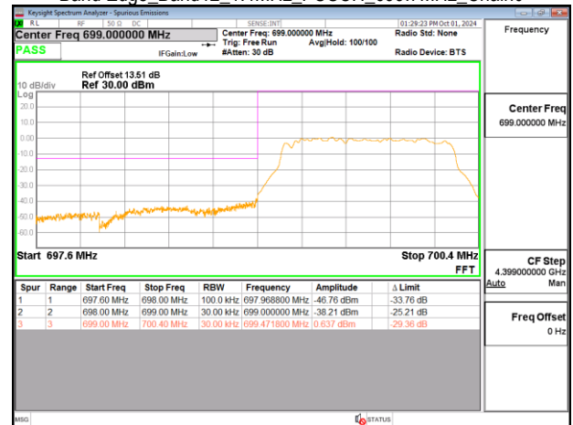
Band Edge_Band12_1.4MHz_PUSCH_699.7MHz_Chain0
