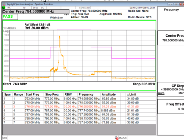
Band Edge_Band13_10MHz_PUSCH_782MHz_Chain0
