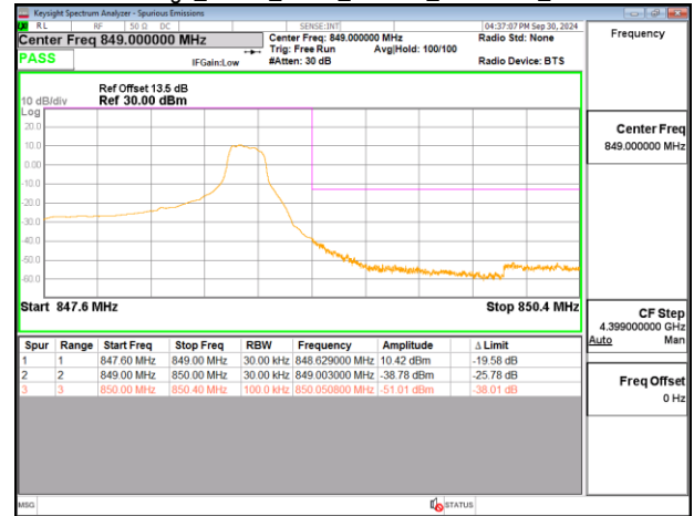
Band Edge_Band5_5MHz_PUSCH_846.5MHz_Chain0
