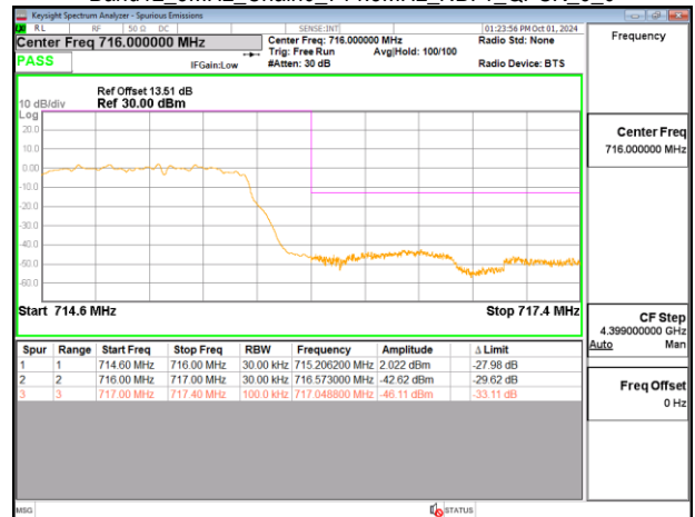
Band12_3MHz_Chain0_714.5MHz_NBI 1_QPSK_6_0
