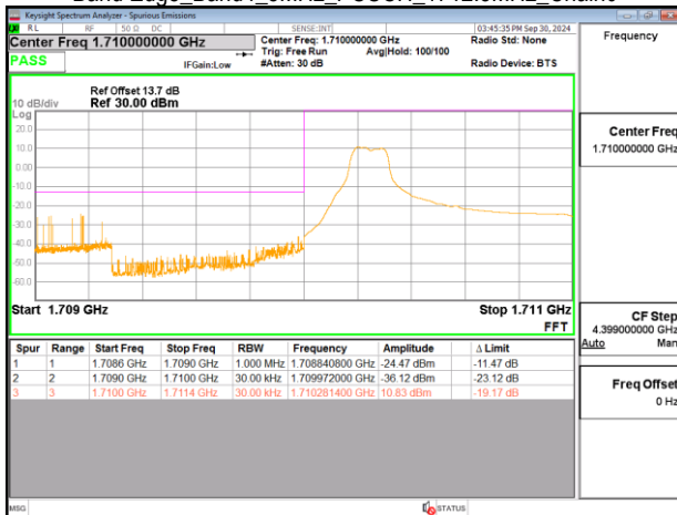
Band Edge_Band4_5MHz_PUSCH_1712.5MHz_Chain0
