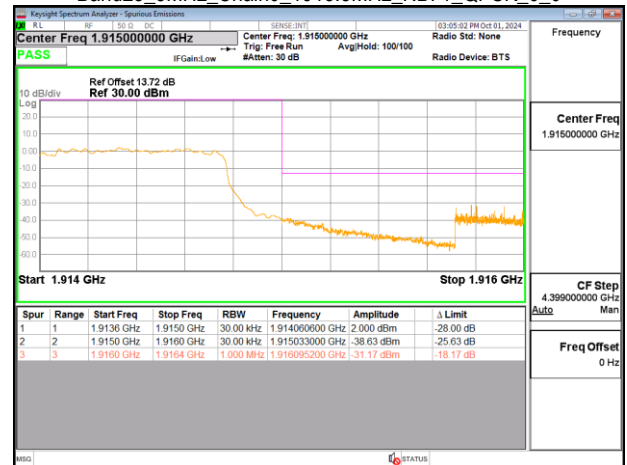
Band25_3MHz_Chain0_1913.5MHz_NBI 1_QPSK 6_0
