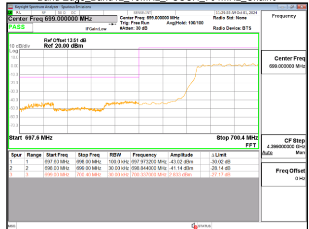
Band Edge_Band12_10MHz_PUSCH_704MHz_Chain0
