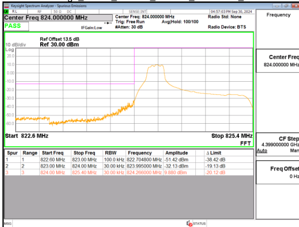
Band Edge_Band5_1.4MHz_PUSCH_824.7MHz_Chain0
