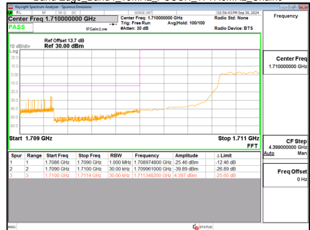
Band Edge_Band4_15MHz_PUSCH_1717.5MHz_Chain0
