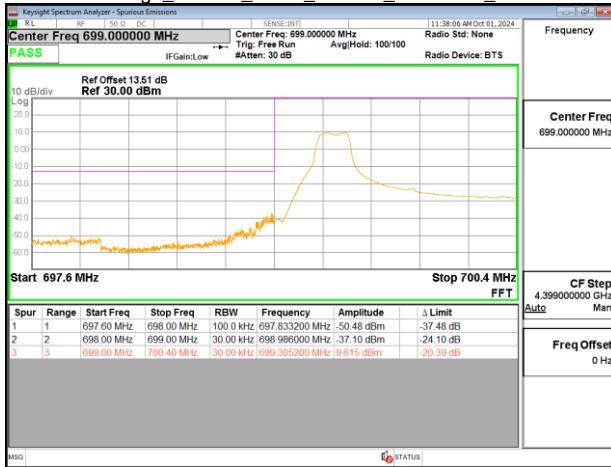
Band Edge_Band12_5MHz_PUSCH_701.5MHz_Chain0
