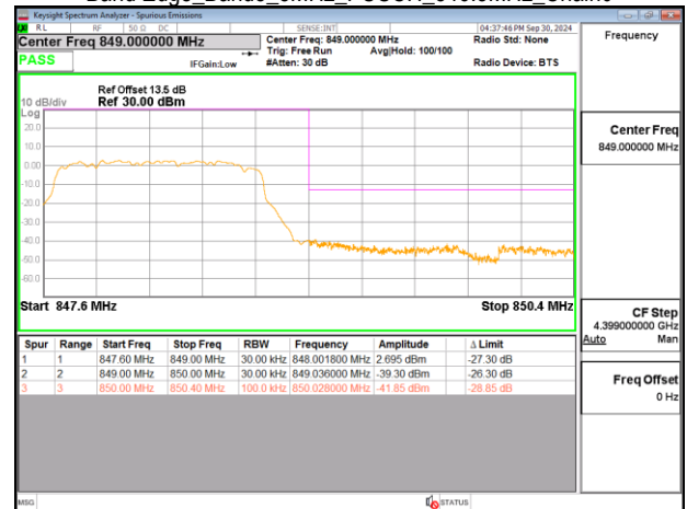
Band Edge_Band5_5MHz_PUSCH_846.5MHz_Chain0
