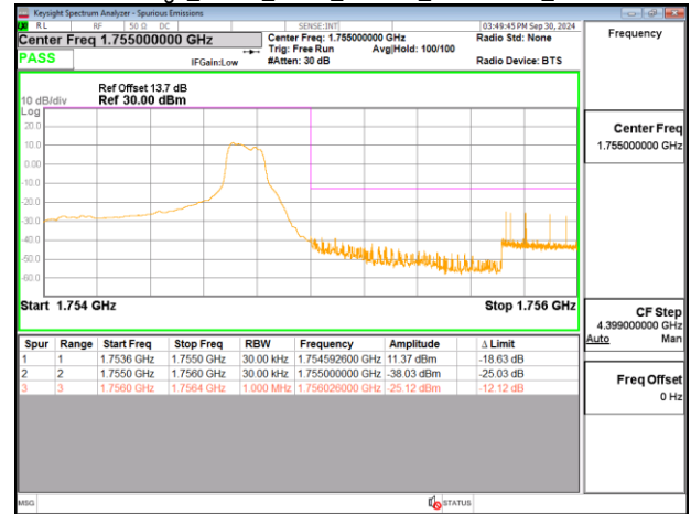
Band Edge_Band4_5MHz_PUSCH_1752.5MHz_Chain0
