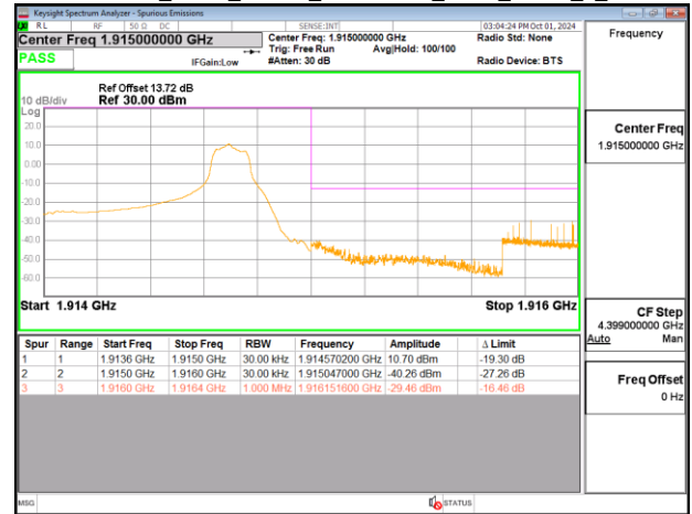
Band25_3MHz_Chain0_1913.5MHz_NBI 1_QPSK 6_0
