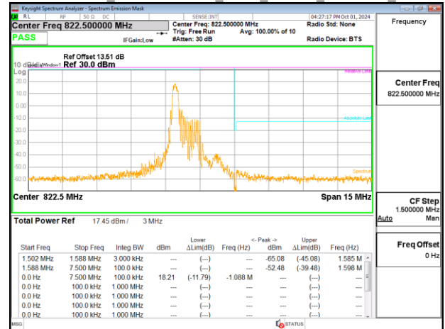
Emission Mask_Band26-Part90s_3MHz_PUSCH_822.5MHz_Chain0
