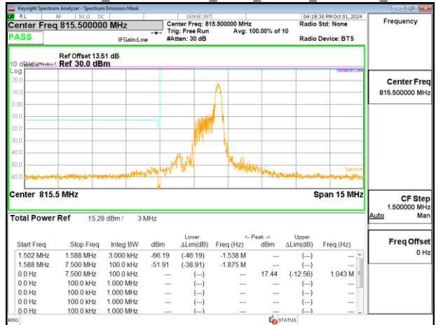
Emission Mask_Band26-Part90s_3MHz_PUSCH_815.5MHz_Chain0
