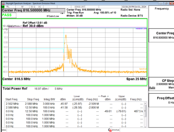
Emission Mask_Band26-Part90s_5MHz_PUSCH_816.5MHz_Chain0
