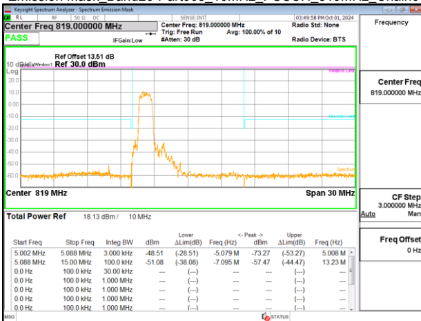
Emission Mask_Band26-Part90s_10MHz_PUSCH_819MHz_Chain0
