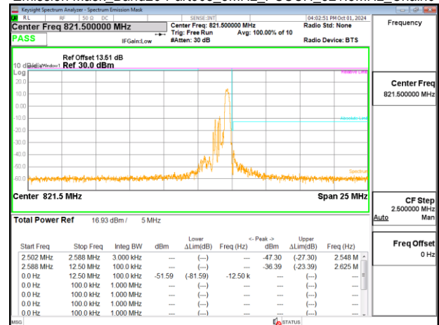
Emission Mask_Band26-Part90s_5MHz_PUSCH_821.5MHz_Chain0
