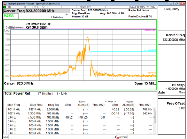
Emission Mask_Band26-Part90s_1.4MHz_PUSCH_823.3MHz_Chain0
