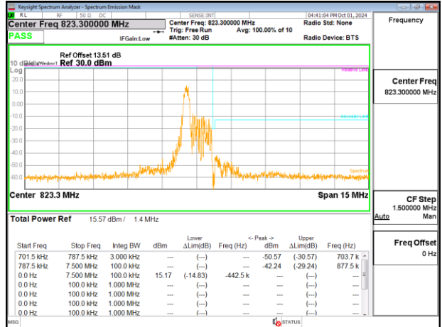
Emission Mask_Band26-Part90s_1.4MHz_PUSCH_823.3MHz_Chain0
