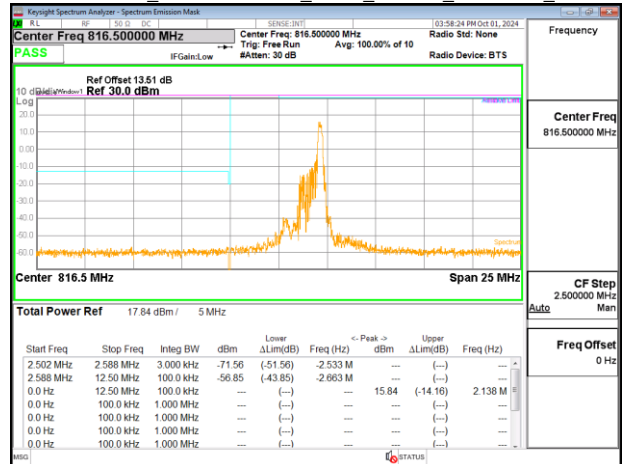
Emission Mask_Band26-Part90s_5MHz_PUSCH_816.5MHz_Chain0
