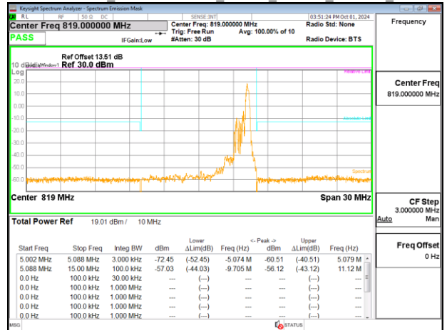
Emission Mask_Band26-Part90s_10MHz_PUSCH_819MHz_Chain0
