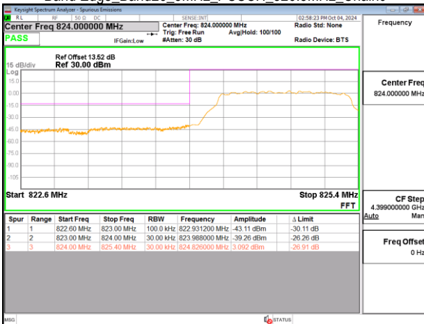
Band Edge_Band26_5MHz_PUSCH_826.5MHz_Chain0
