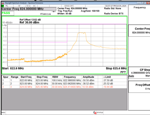
Band Edge_Band26_5MHz_PUSCH_826.5MHz_Chain0
