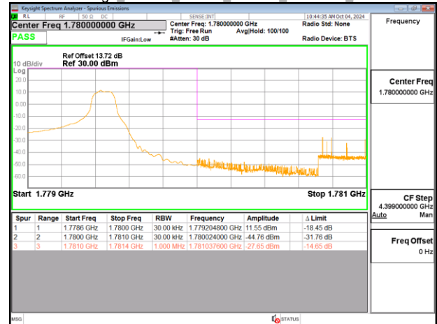
Band Edge_Band66_10MHz_PUSCH_1775MHz_Chain0
