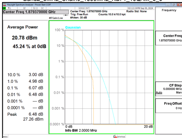
Band2_5MHz_Chain0_1880MHz_NBI 1_16QAM_6_0
