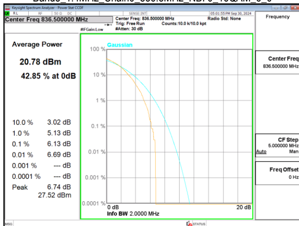
Band5_1.4MHz_Chain0_836.5MHz_NBI 0_16QAM_6_0
