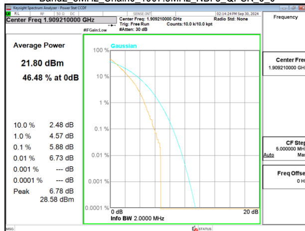
Band2_5MHz_Chain0_1907.5MHz_NBI 3_QPSK_6_0
