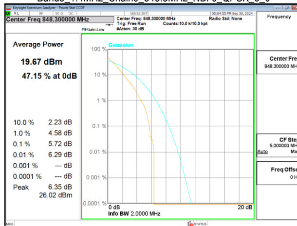
Band5_1.4MHz_Chain0_848.3MHz_NBI 0_QPSK_6_0
