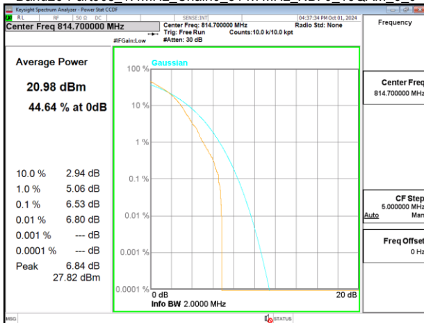
Band26-Part90s_1.4MHz_Chain0_814.7MHz_NBI 0_16QAM_6_0
