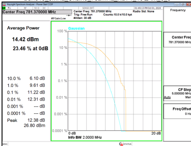
Band13_5MHz_Chain0_782MHz_NBI 1_16QAM_6_0
