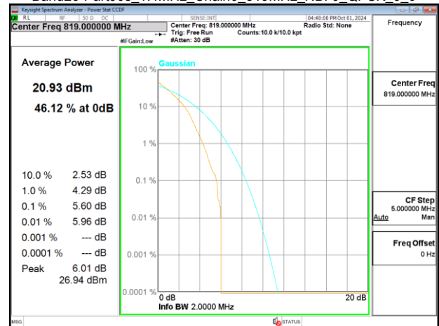
Band26-Part90s_1.4MHz_Chain0_819MHz_NBI 0_QPSK_6_0
