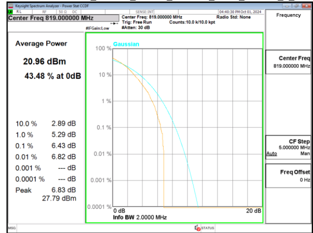
Band26-Part90s_1.4MHz_Chain0_819MHz_NBI 0_QPSK_6_0
