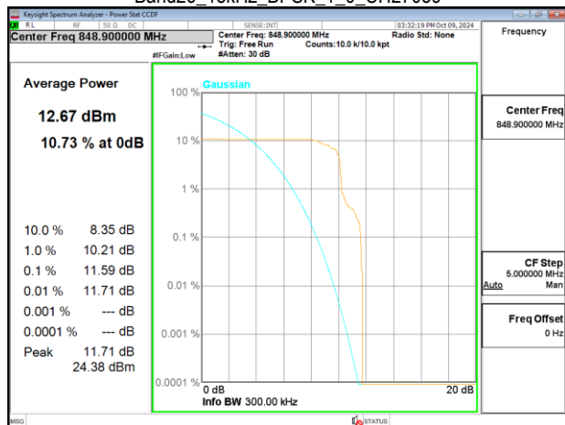
Band26_15kHz_BPSK_1_0_CH27039
