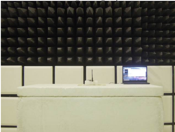
Cat-M1_Radiated_Setup
