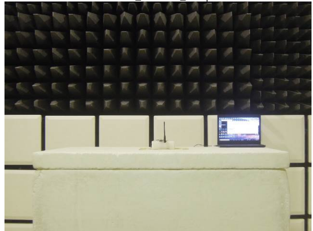
NB-IoT_Radiated_Setup
