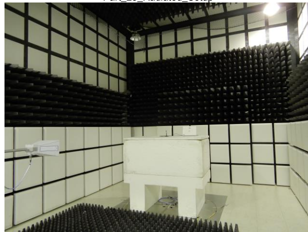
Part_25_Radiated_Setup
