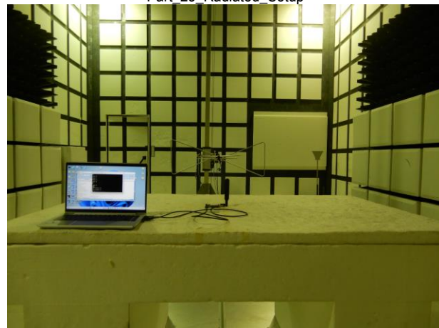
Part_25_Radiated_Setup
