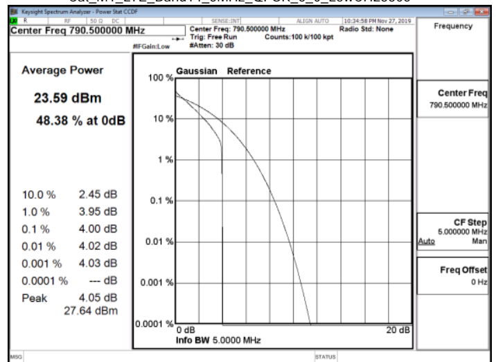
Cat_M1_LTE_Band14_5MHz_QPSK_6_0_LowCH23305
