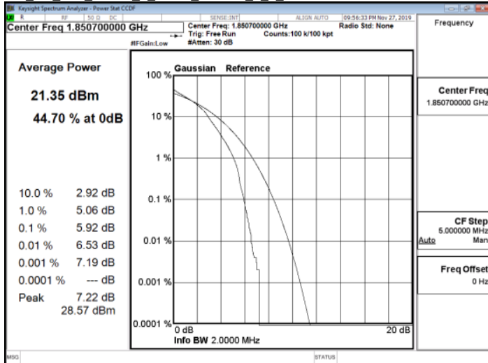
Cat_M1_LTE_Band2_1_4MHz_QPSK_6_0_LowCH18607-1850.7
