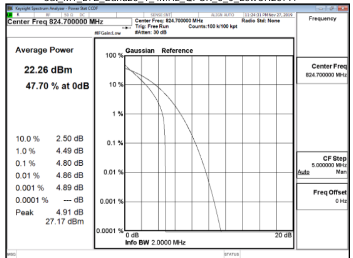
Cat_M1_LTE_Band26_1_4MHz_QPSK_6_0_LowCH26797
