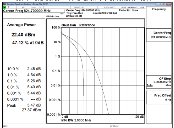
Cat_M1_LTE_Band5_1_4MHz_QPSK_6_0_LowCH20407-824.7
