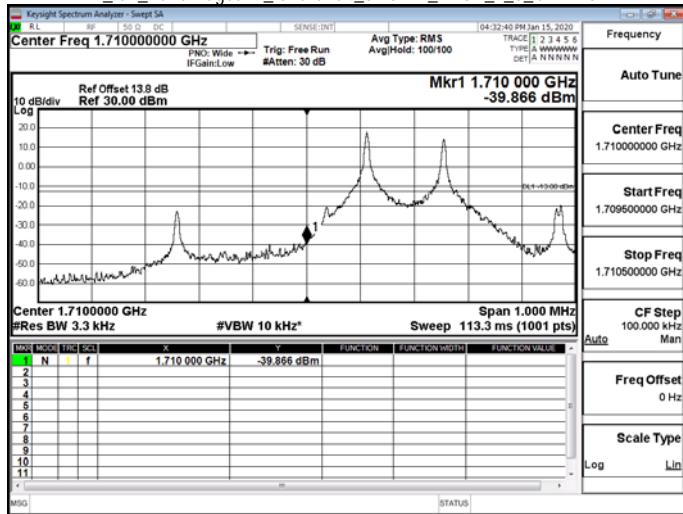
NB_IoT_Band Edge\NB_IoT\Band4_3.75kHz_BPSK_1_47_CH20398
