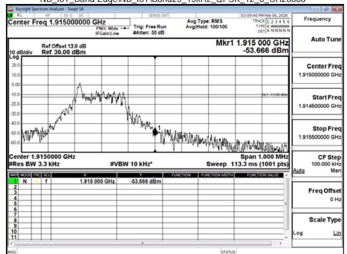
NB_IoT_Band Edge\NB_IoT\Band25_15kHz_QPSK_12_0_CH26688
