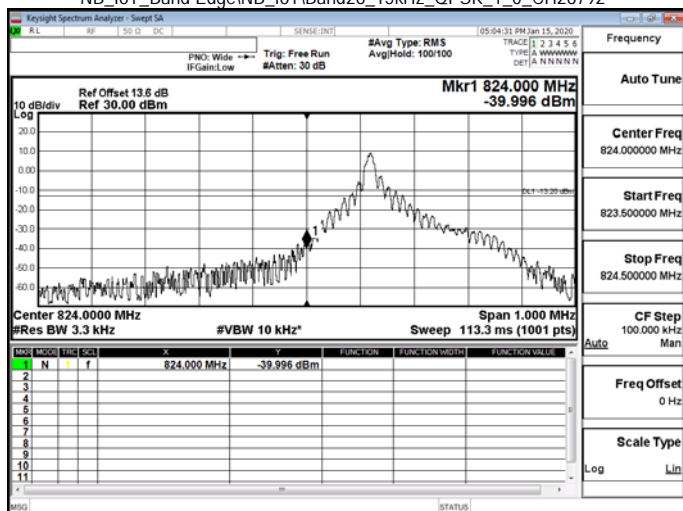
NB_IoT_Band Edge\NB_IoT\Band26_15kHz_QPSK_1_0_CH26792
