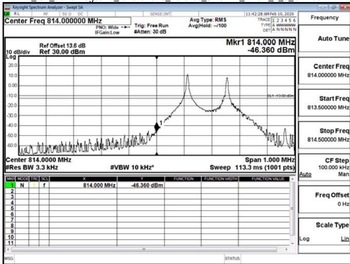
NB_IoT_Band Edge/NB_IoTBand26_Part90s_3.75kHz_BPSK_1_47_CH26788
