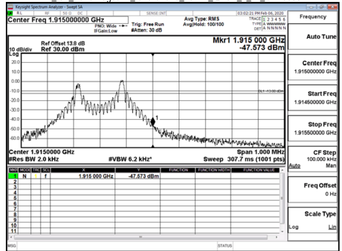
NB_IoT_Band Edge\NB_IoT\Band25_15kHz_QPSK_12_0_CH26042
