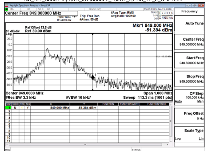
NB_IoT_Band Edge\NB_IoT\Band26_15kHz_QPSK_12_0_CH27038
