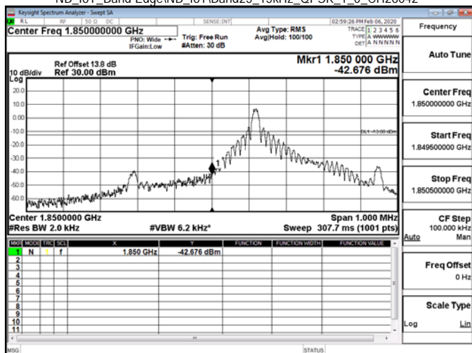
NB_IoT_Band Edge\NB_IoT\Band25_15kHz_QPSK_1_0_CH26042
