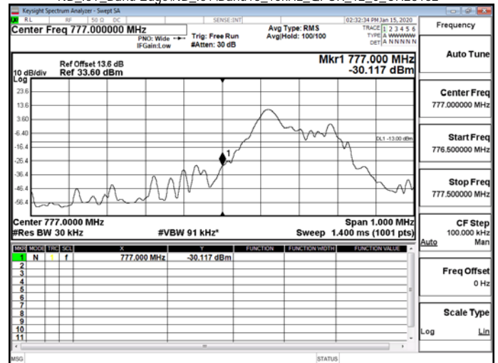
NB_IoT_Band Edge\NB_IoT\Band13_15kHz_QPSK_12_0_CH23278
