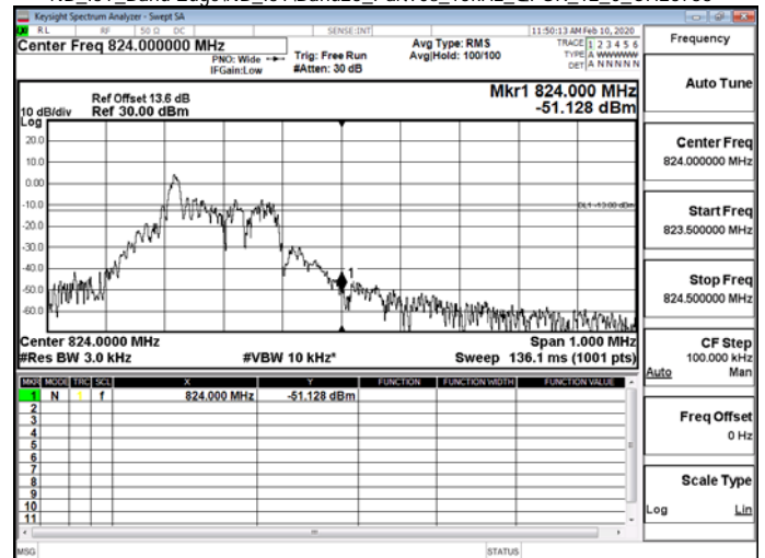
NB_IoT_Band Edge/NB_IoTBand26_Part90s_15kHz_QPSK_12_0_CH26788
