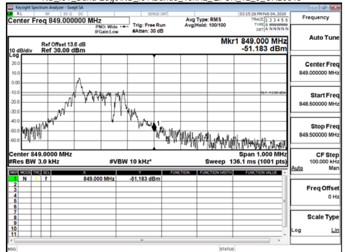
NB_IoT_Band Edge\NB_IoT\Band5_15kHz_QPSK_12_0_CH20648
