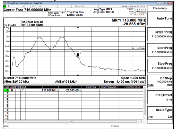
NB_IoT_Band Edge\NB_IoT\Band17_15kHz_QPSK_12_0_CH23732
