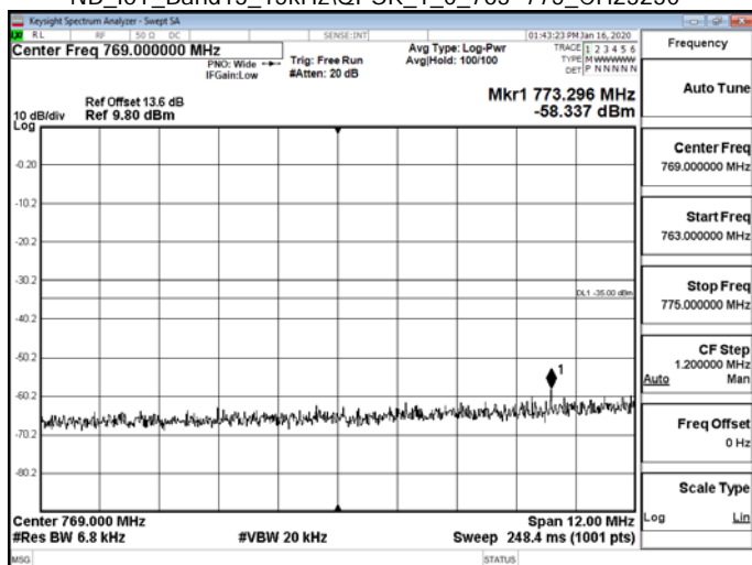
NB_IoT_Band13_15kHz/QPSK_1_0_763-775_CH23230
