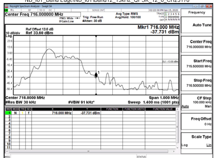
NB_IoT_Band Edge\NB_IoT\Band12_15kHz_QPSK_12_0_CH23178
