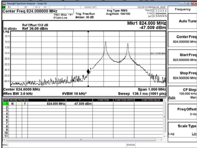
NB_IoT_Band Edge\NB_IoT\Band5_3.75kHz_BPSK_1_47_CH20648
