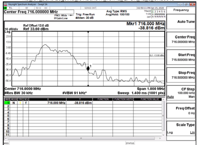
NB_IoT_Band Edge\NB_IoT\Band17_15kHz_QPSK_12_0_CH23848
