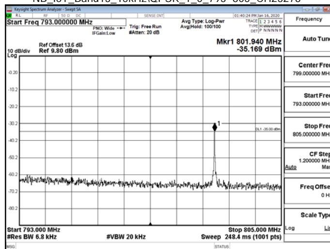
NB_IoT_Band13_15kHz/QPSK_1_0_793-805_CH23278
