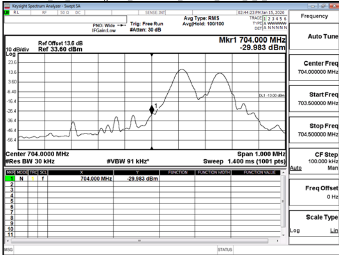
NB_IoT_Band Edge\NB_IoT\Band17_3.75kHz_BPSK_1_47_CH23848
