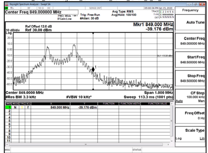
NB_IoT_Band Edge\NB_IoT\Band26_15kHz_QPSK_12_0_CH26792
