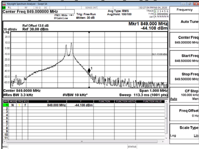
NB_IoT_Band Edge\NB_IoT\Band5_15kHz_QPSK_1_0_CH20402
