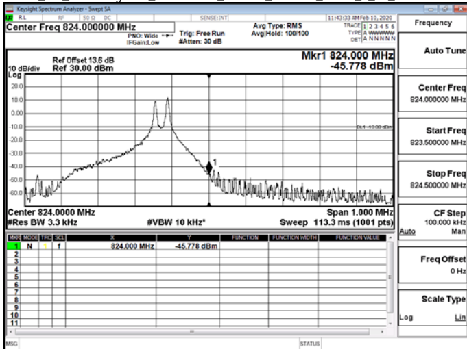
NB_IoT_Band Edge/NB_IoTBand26_Part90s_15kHz_QPSK_1_0_CH26692
