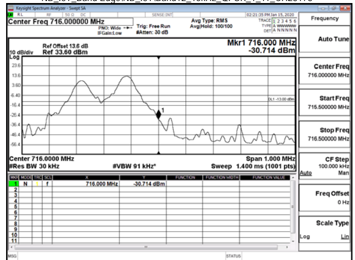
NB_IoT_Band Edge\NB_IoT\Band12_15kHz_QPSK_12_0_CH23012
