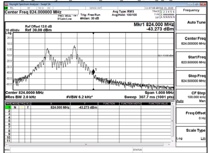
NB_IoT_Band Edge/NB_IoTBand26_Part90s_15kHz_QPSK_12_0_CH26692
