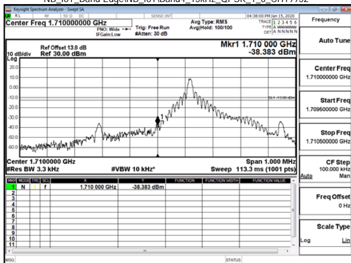
NB_IoT_Band Edge\NB_IoT\Band4_15kHz_QPSK_1_0_CH19952
