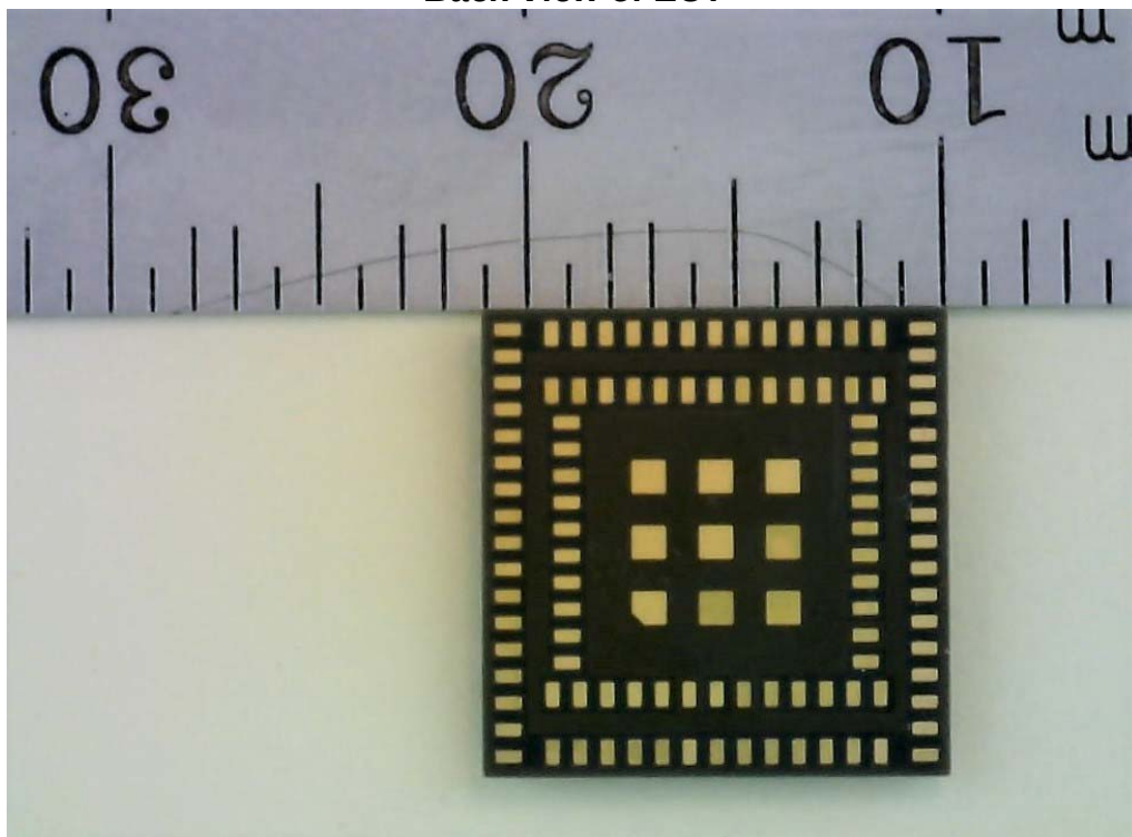
Back View of EUT
