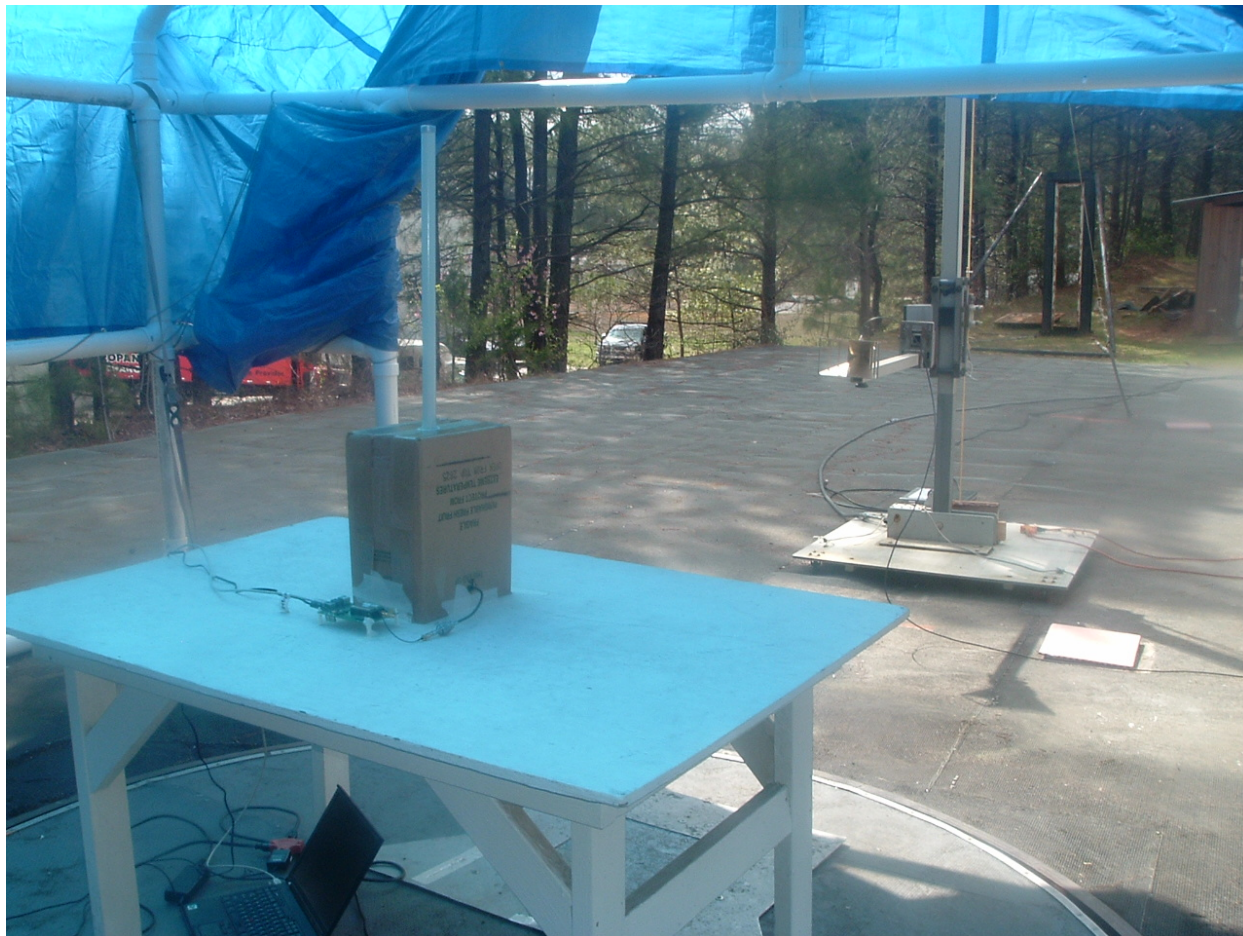
Photo 5. Above 1GHz Test setup at 3 meter
