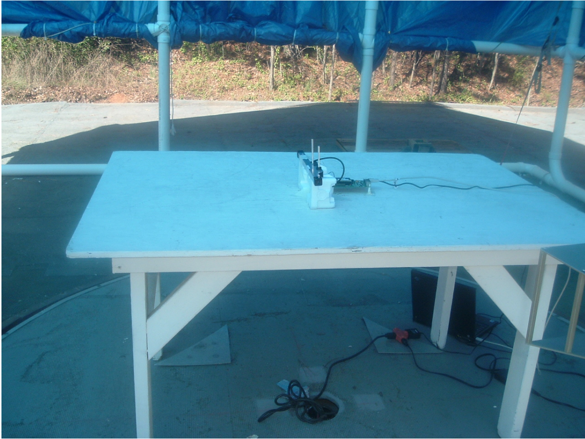
Photo 2. Front View of EUT Yagi antenna
