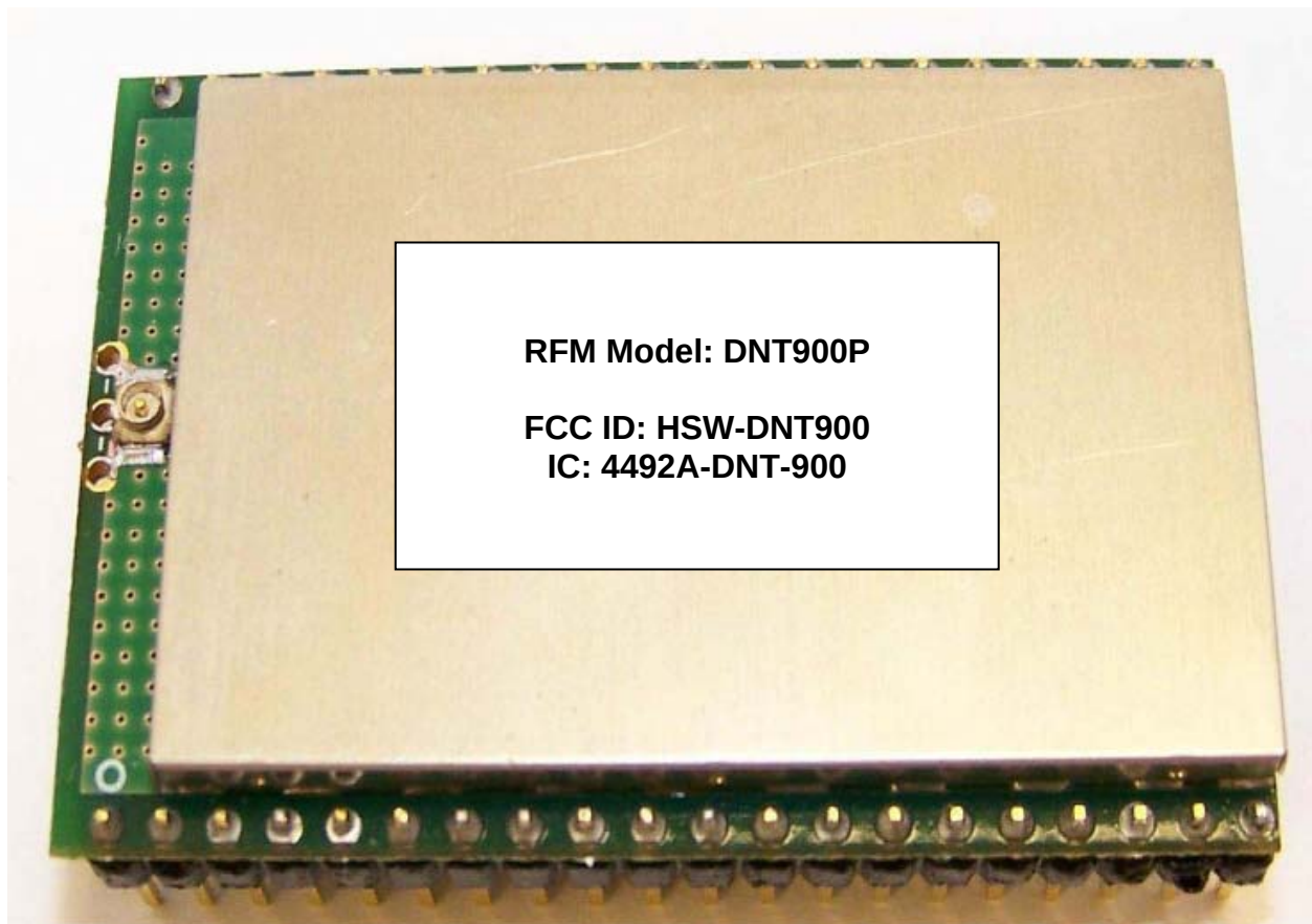
Photo 2. Model DNT900P
