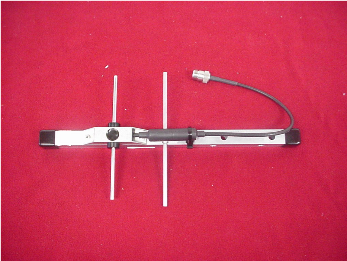
Photo 2 Yagi Antenna
