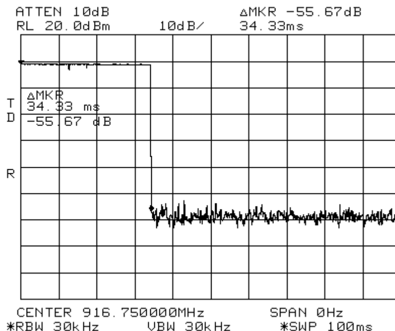
Figure 7.2.3.2-1: Duty Cycle Timing Diagram
