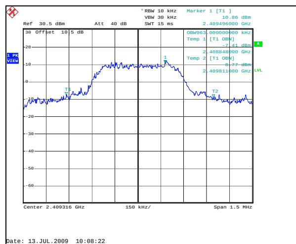
Figure 7.5.4-16: 99% Bandwidth Low Channel – 500 kbps
