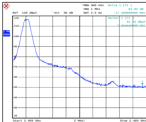
Figure 7.6.1.2-4: Upper Band-edge Vpol (Hopping) – Dipole
