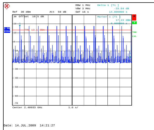
Figure 7.5.3-4: Repetition – 115.2 kbps (12 * 18.3ms = 219.6ms)
