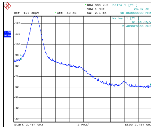
Figure 7.6.1.2-2: Upper Band-edge Vpol – Dipole
