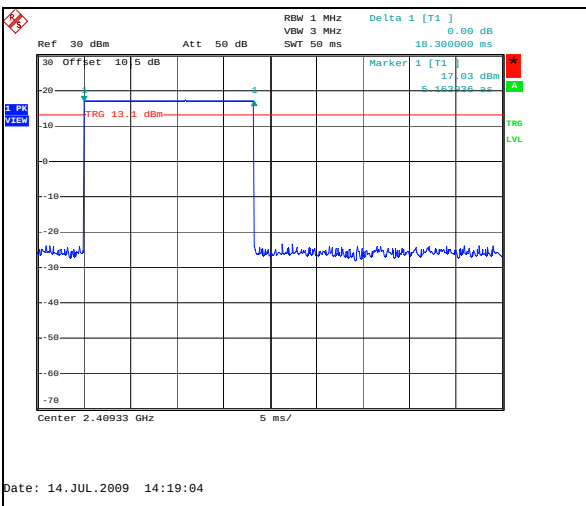
Figure 7.5.3-3: Dwell Time – 115.2 kbps (18.3ms)
