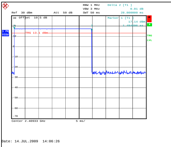
Figure 7.5.3-1: Dwell Time – 38.4 kbps (28.8ms)
