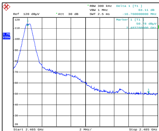
Figure 7.6.1.2-3: Upper Band-edge Hpol (Hopping) – Dipole
