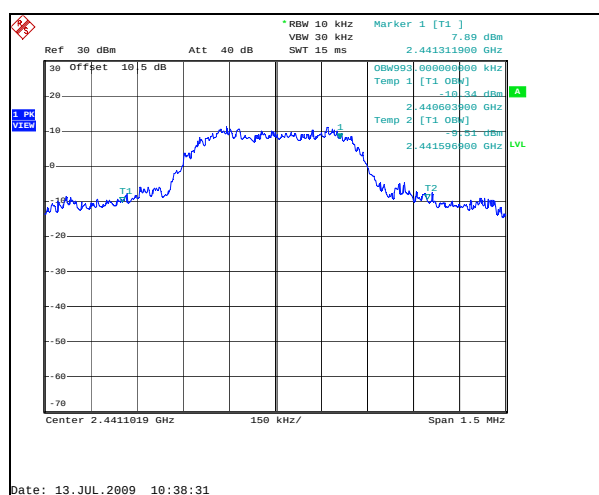
Figure 7.5.4-20: 99% Bandwidth Mid Channel – 500 kbps
