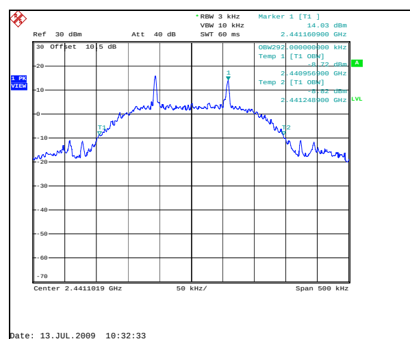
Figure 7.5.4-18: 99% Bandwidth Mid Channel – 115.2 kbps
