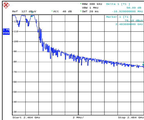
Figure 7.6.1.2-2: Upper Band-edge Vpol – Dipole
