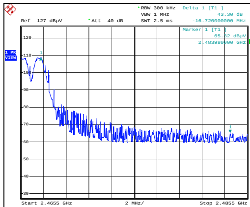
Figure 7.6.1.2-1: Upper Band-edge Hpol – Dipole
