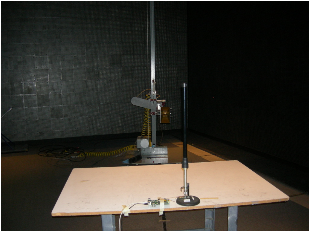
Figure 1: Radiated Emissions – Dipole Antenna
