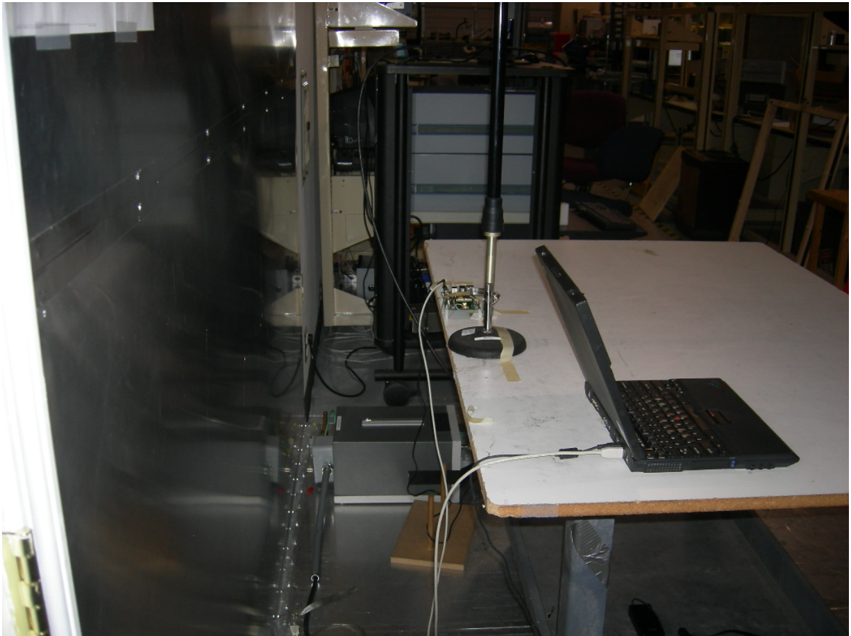
Figure 4: AC Power Line Conducted Emissions – Dipole Antenna
