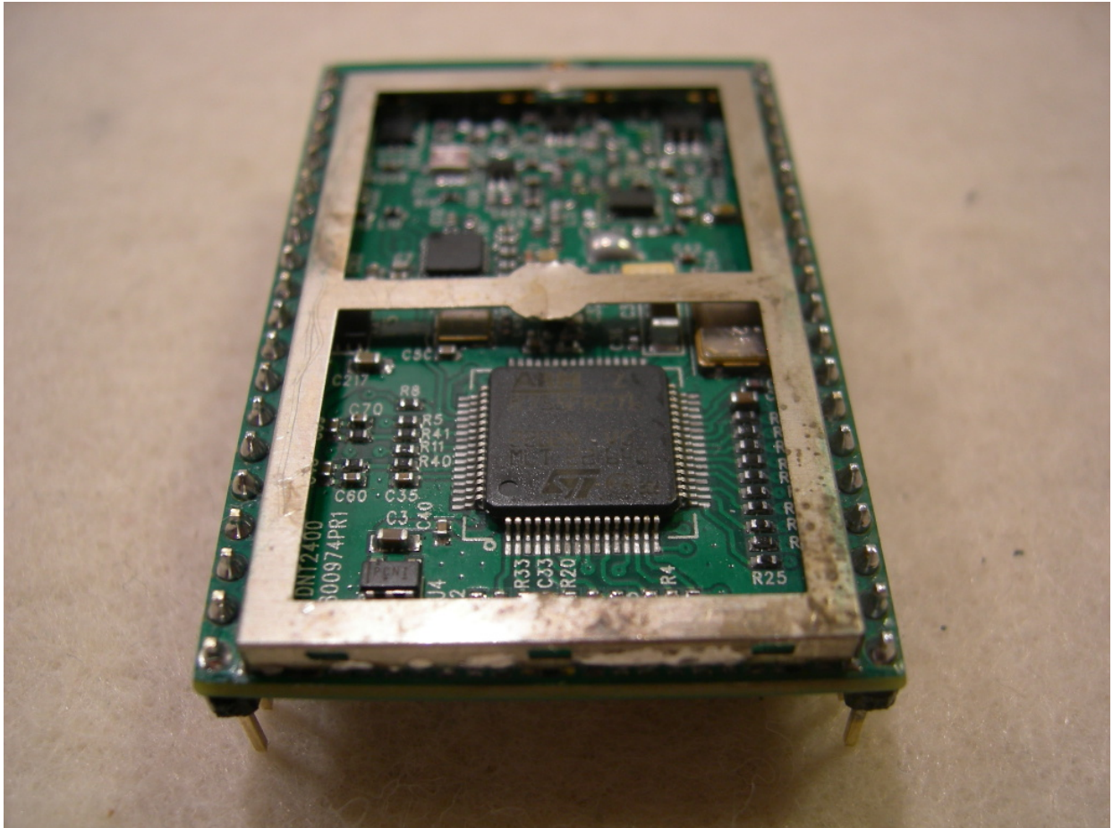
Figure 4: PCB without Shields - Front
