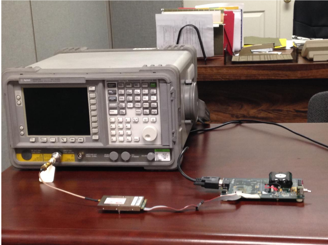
Figure 4. Bench Testing Setup
