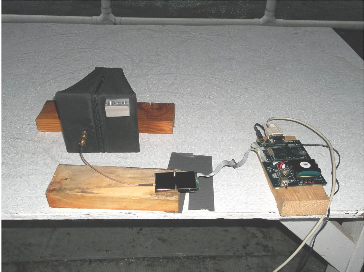
Figure 2. Test configuration
