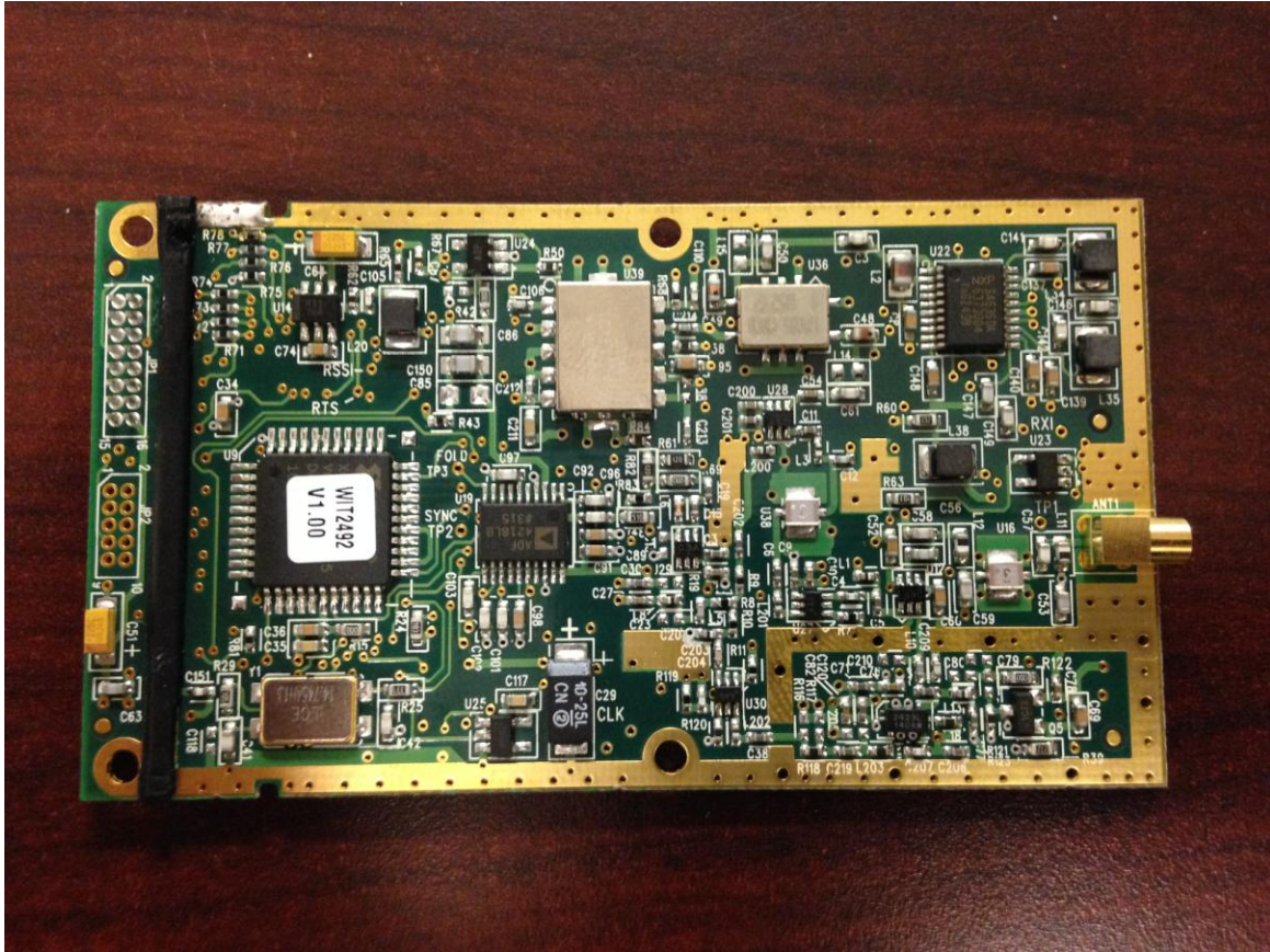
Figure 1. Top, Component Side
