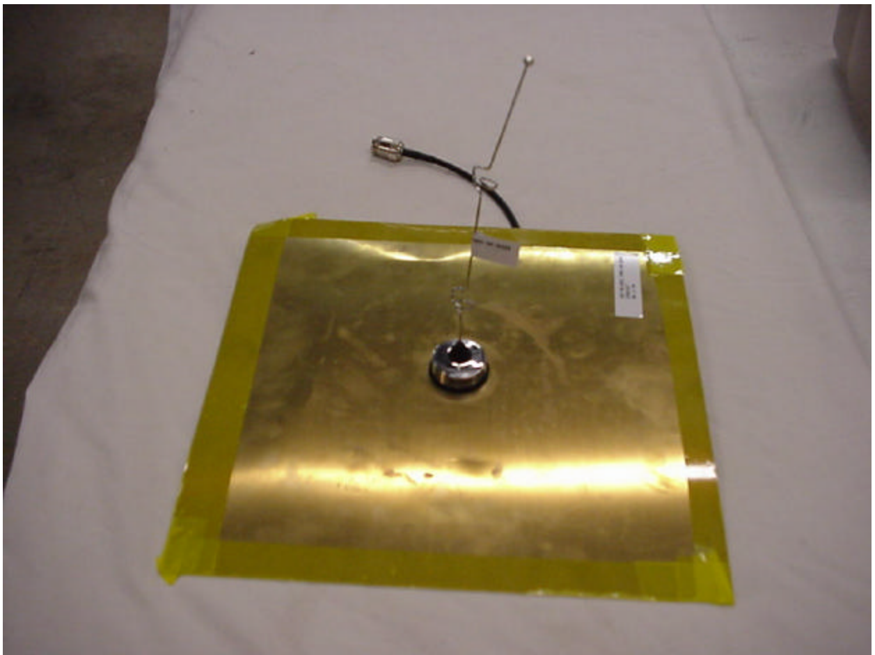
Photo 11. Whip Antenna
