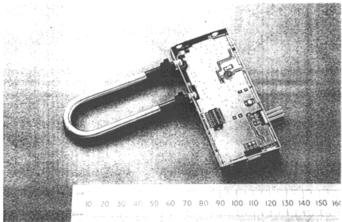
Component side view of transmitter with cover removed
