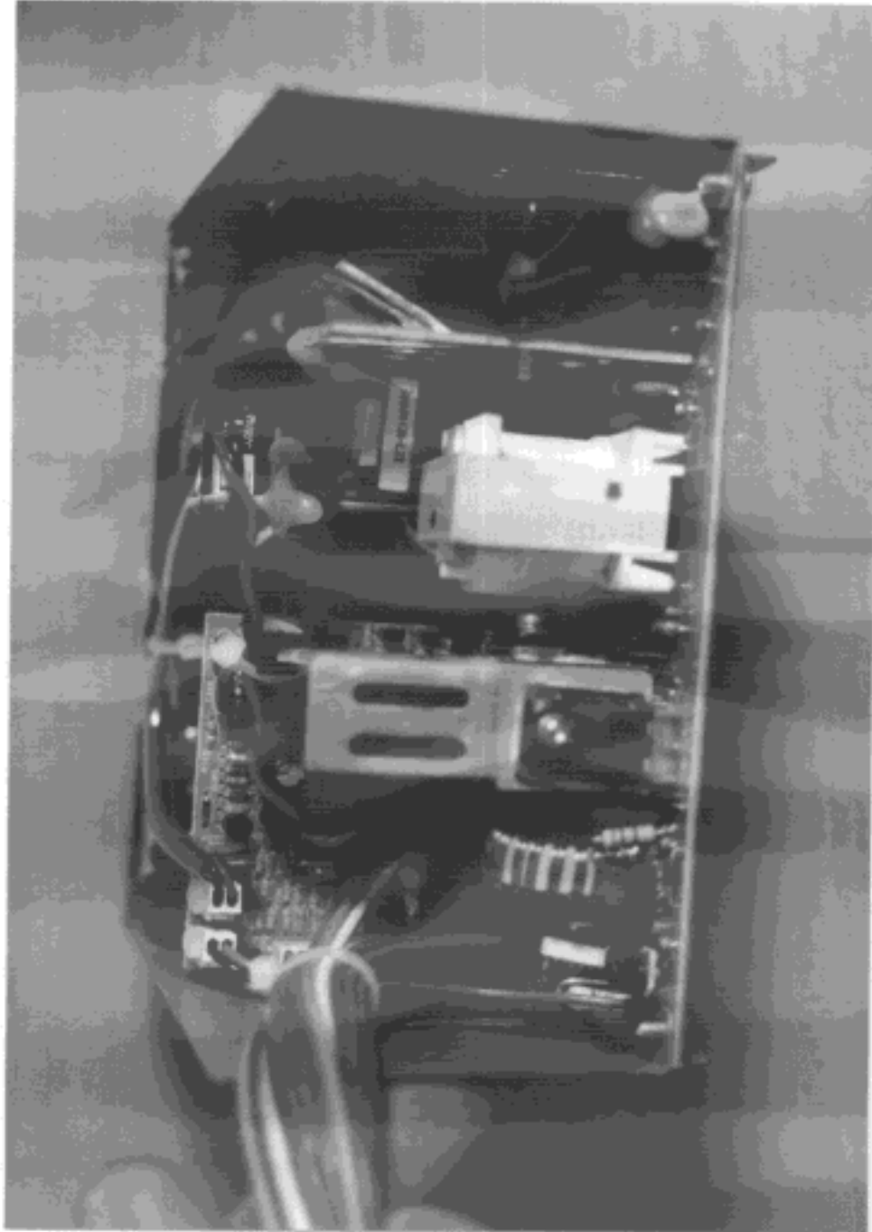
8.4 Power supply Minebea (GS3), opened case, inside view, part two
