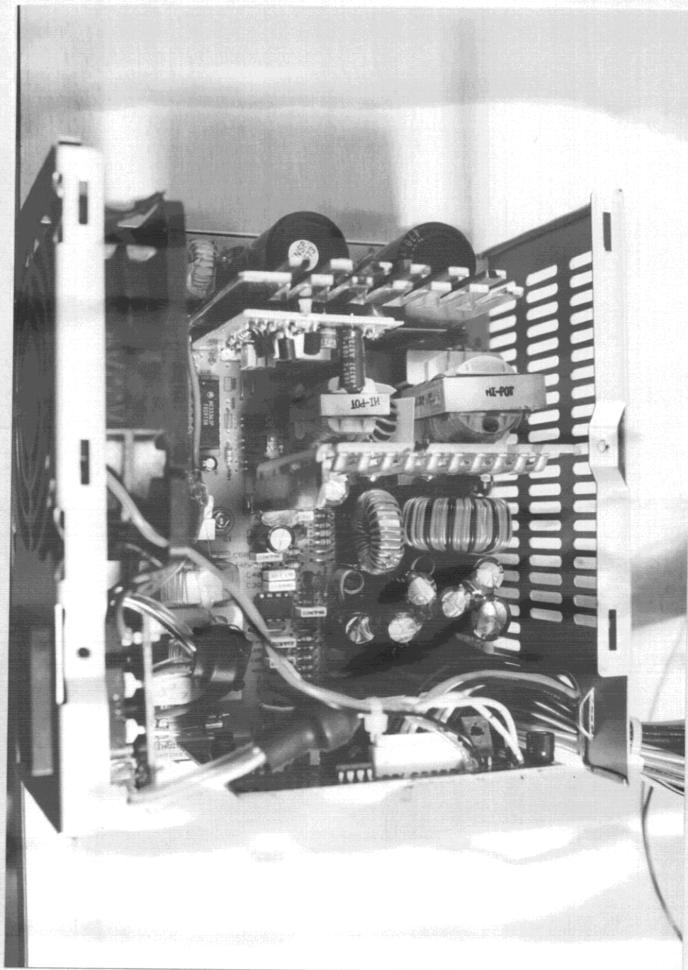
8.7 Power supply ASTEC, opened case, inside view
