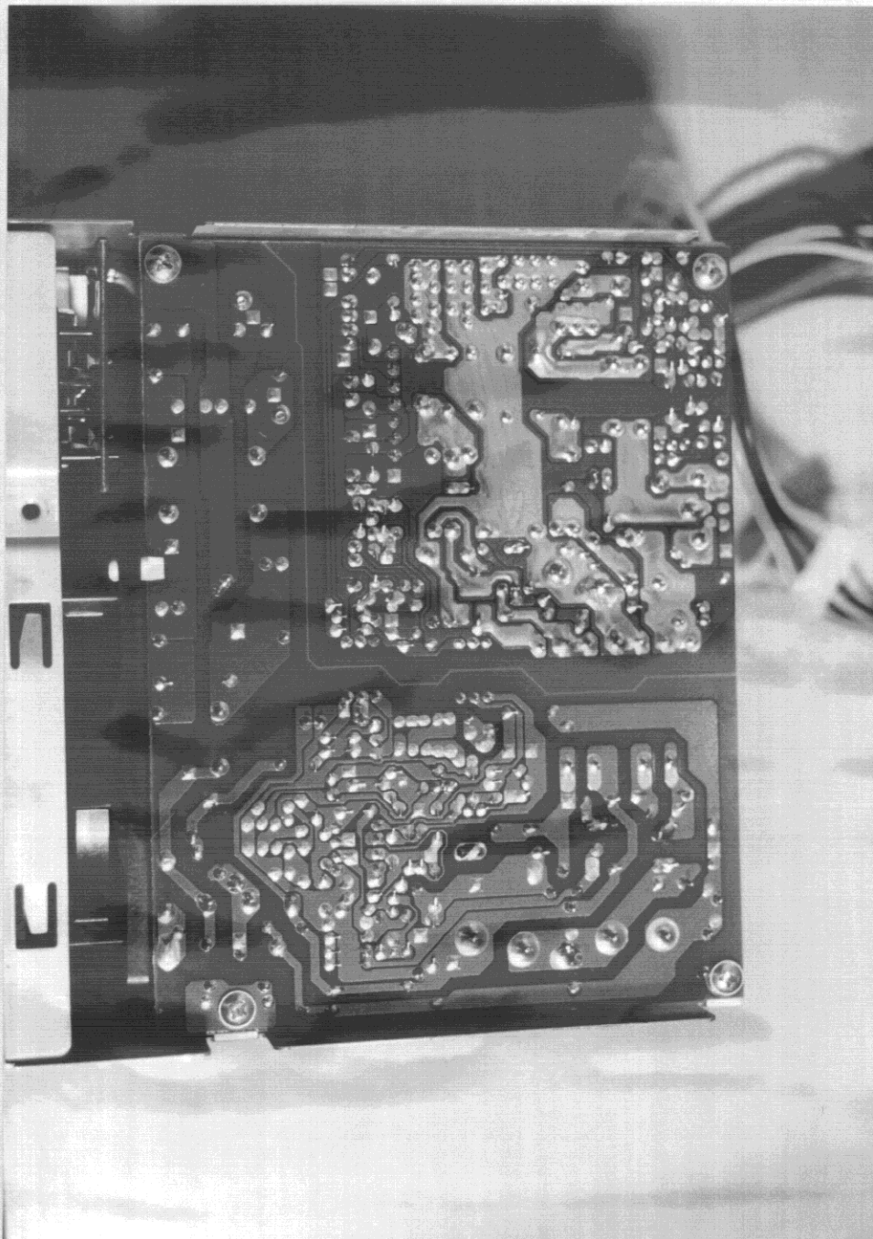
8.5 Power supply Minebea (GS3), opened case, rear side view
