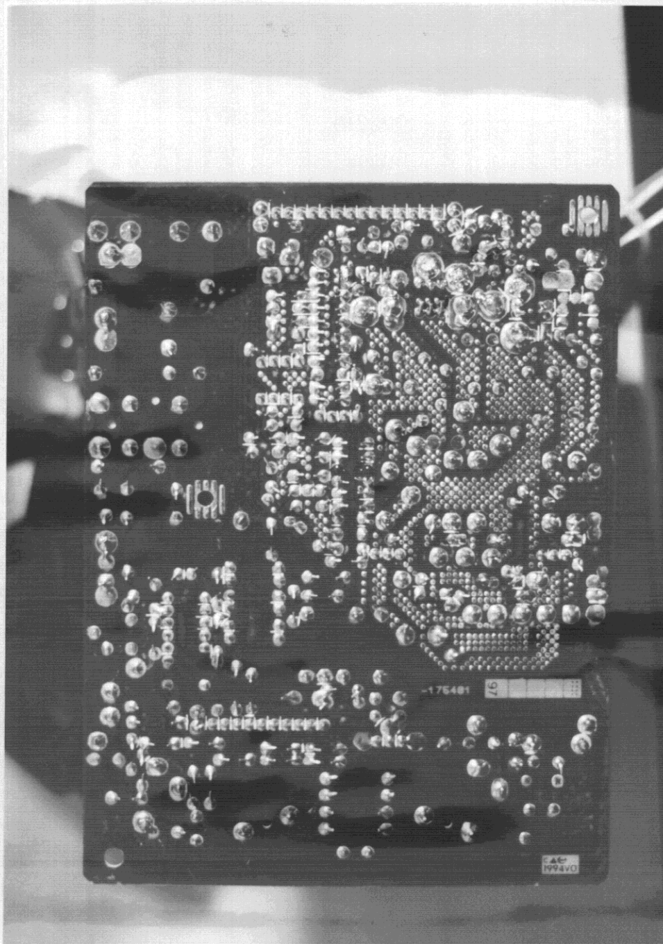
8.8 Power supply ASTEC, opened case, rear side view
