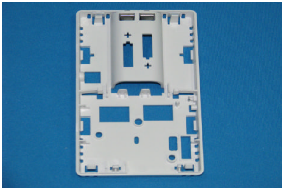
Bottom Cover Internal View
