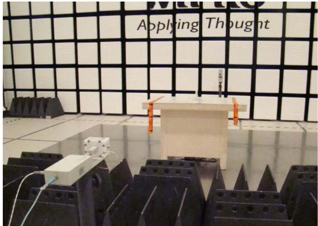
Setup for Radiated Emission
