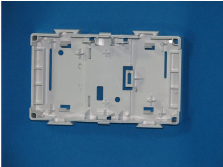
Back cover Internal View
