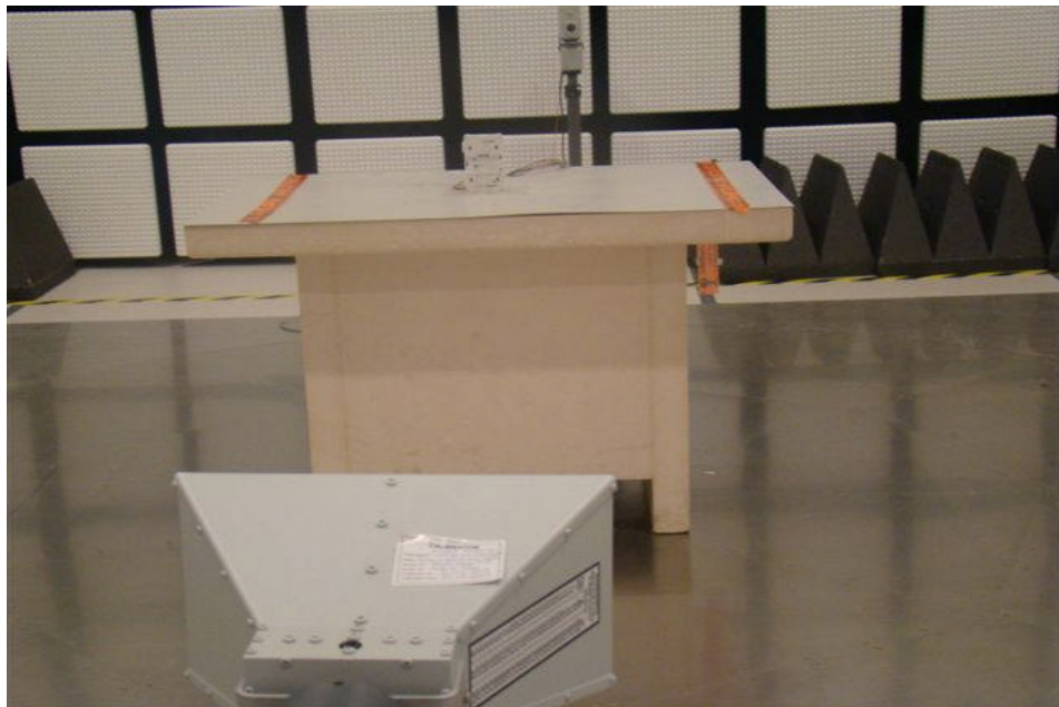
Setup for Radiated Emission
