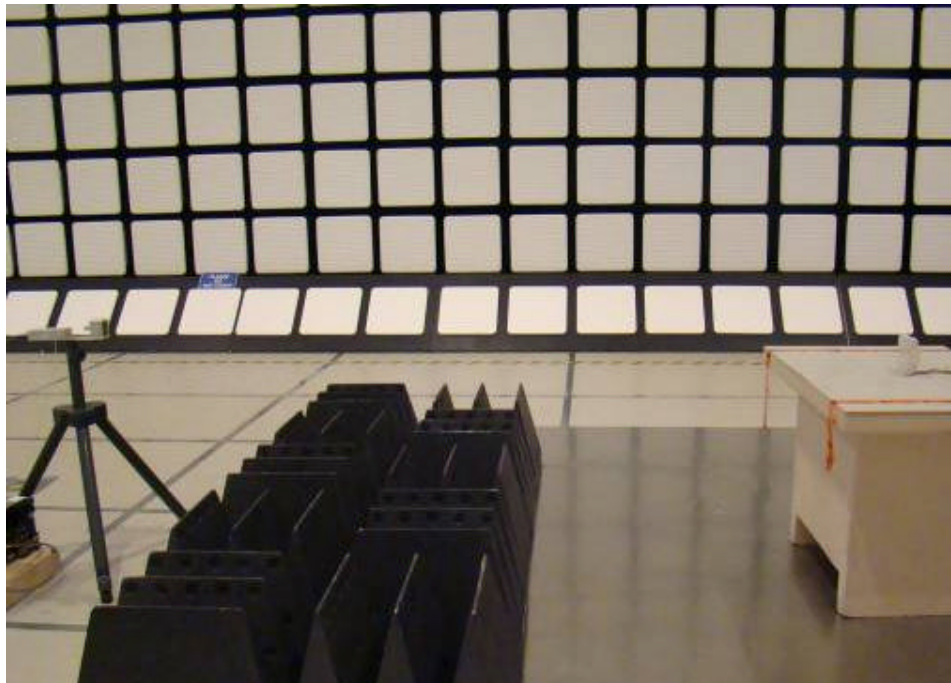
Setup for Radiated Emission
