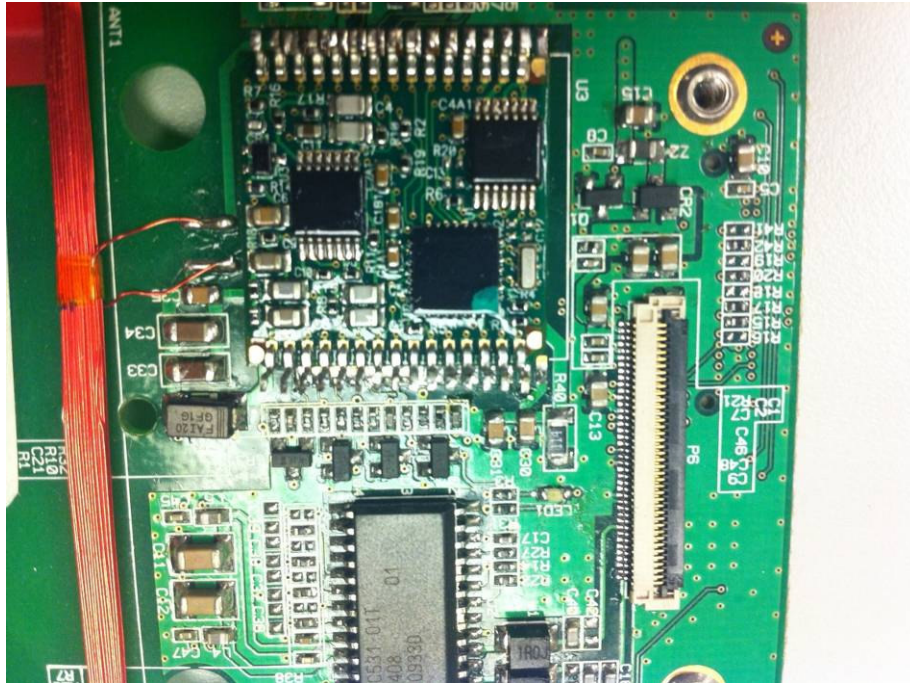
13.56MHz MF RC531 RF Module
