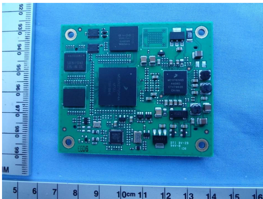
Internal of PCB Front Side
