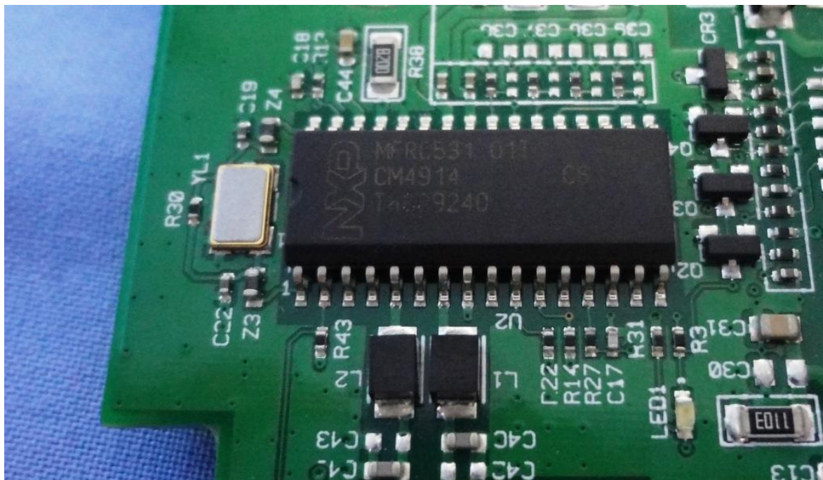
13.56MHz MF RC531 RF Module
