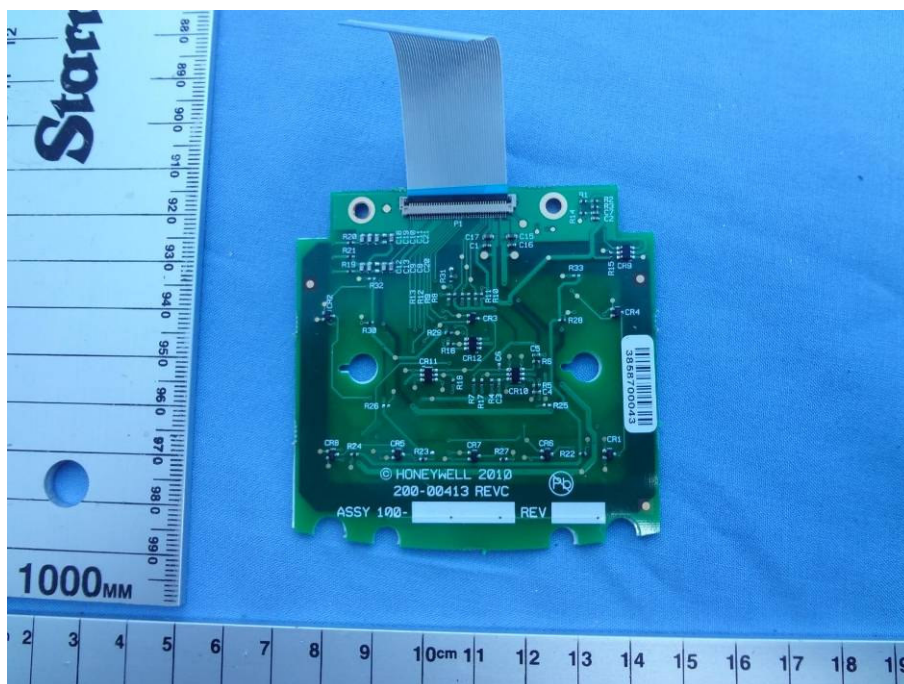
Keypad Back Side
