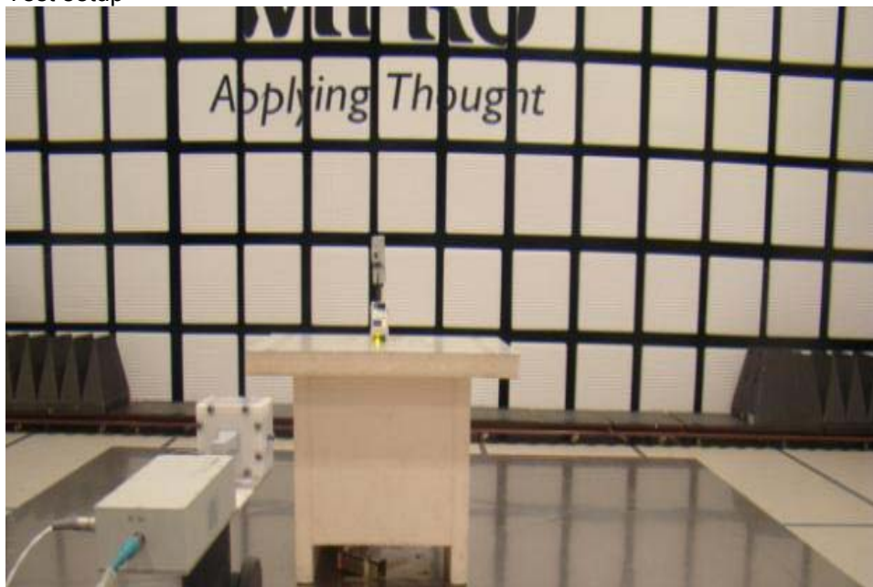
Test setup
