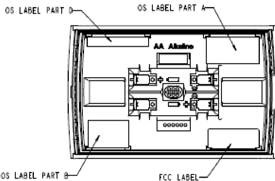
BACK VIEW BEFORE MOUNTING PLATE INSTALLATION
