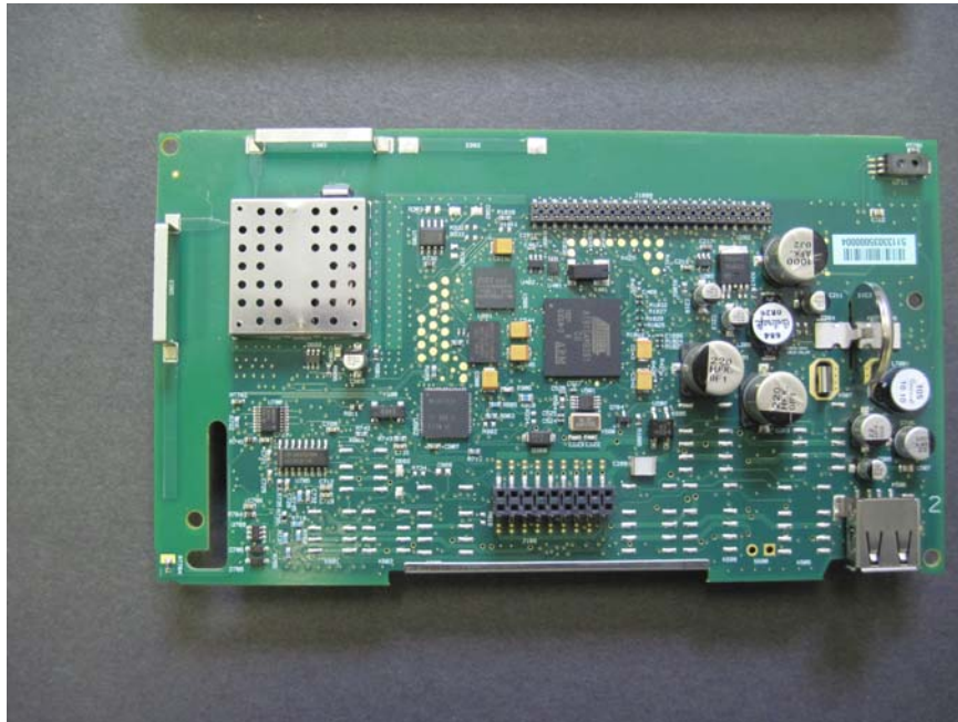
View of RF Board, Shielded
