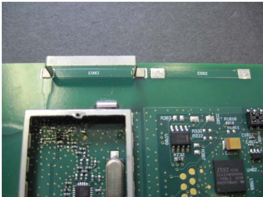
View of RF Section, Unshielded
