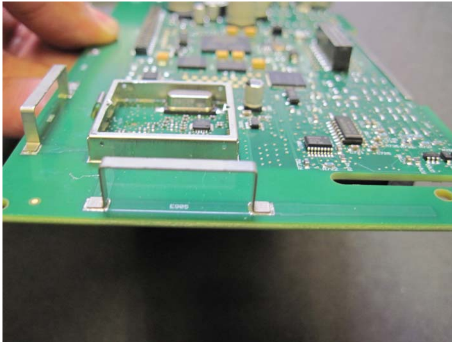
Close-Up of RF Section, Unshielded, View #5
