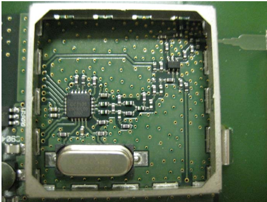
Close-Up of RF Section, Unshielded, View #2
