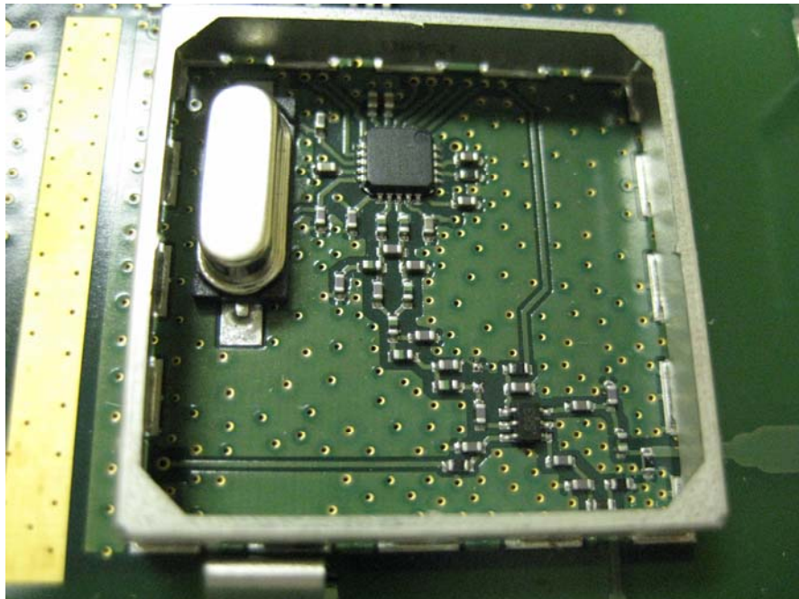
Close-Up of RF Section, Unshielded, View #4
