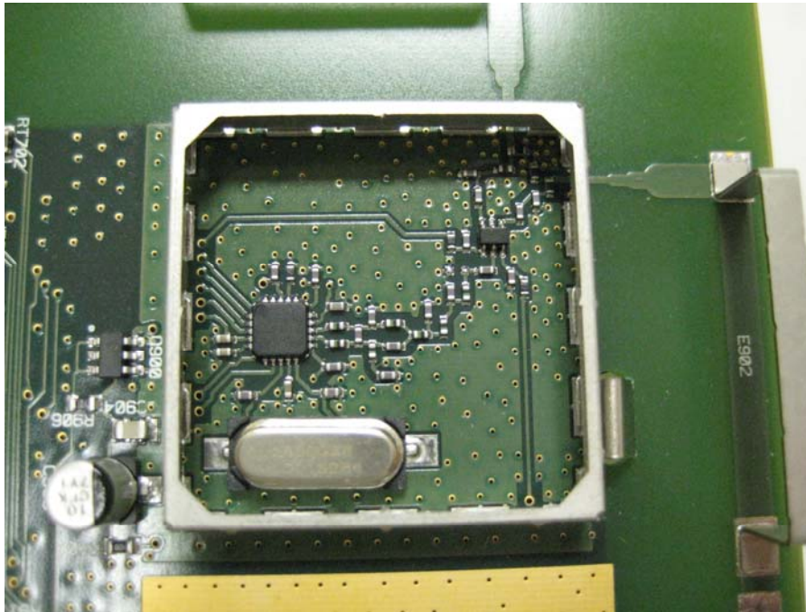
Close-Up of RF Section, Unshielded, View #1
