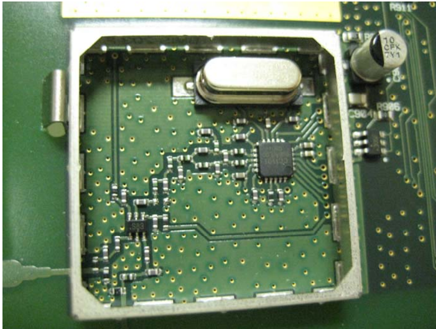
Close-Up of RF Section, Unshielded, View #3
