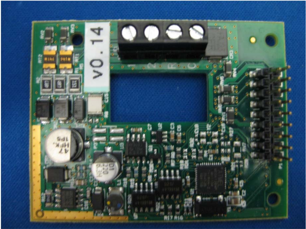
Close up of board removed from wall plate (picture 1)
