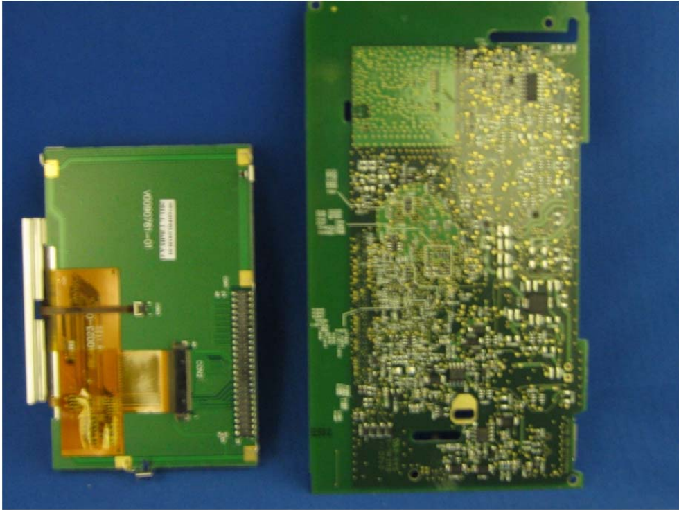
Display removed from board
