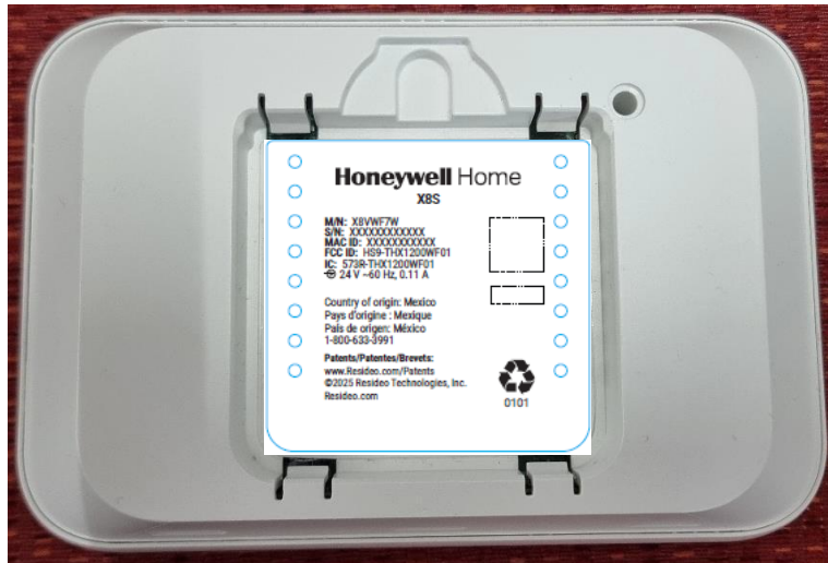
Figure 3 X8VWF7W Label and label location
